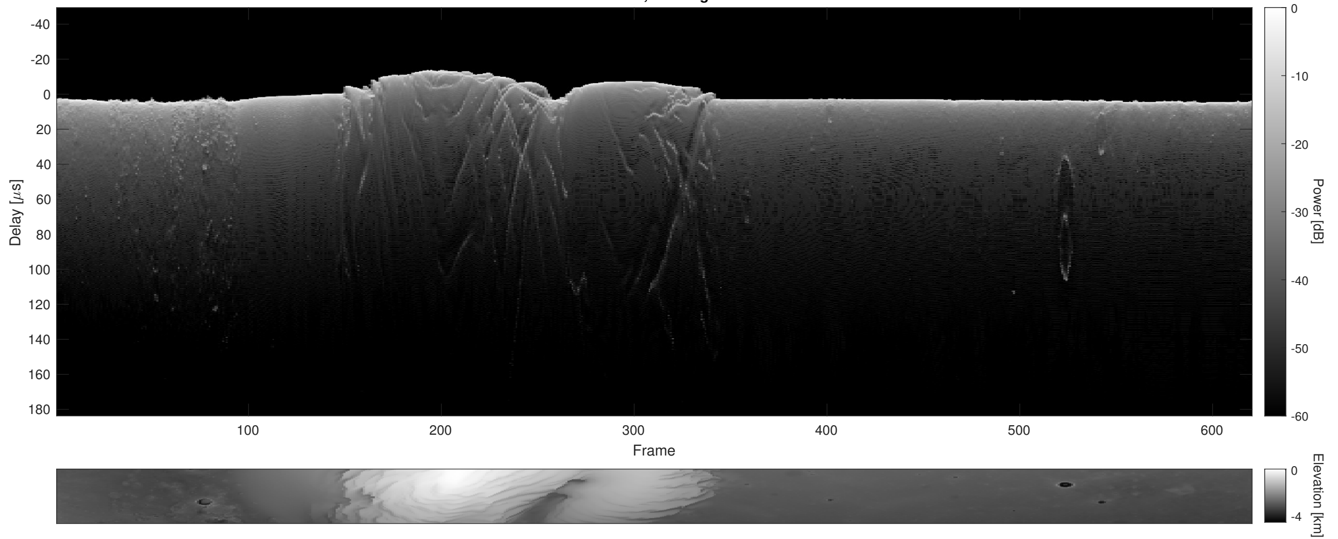
Orbit 7511, Cluttergram
