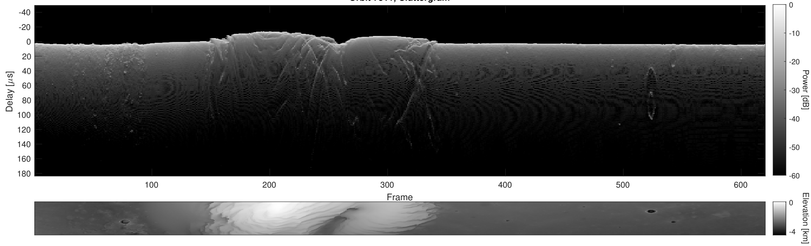
Orbit 7511, Cluttergram
