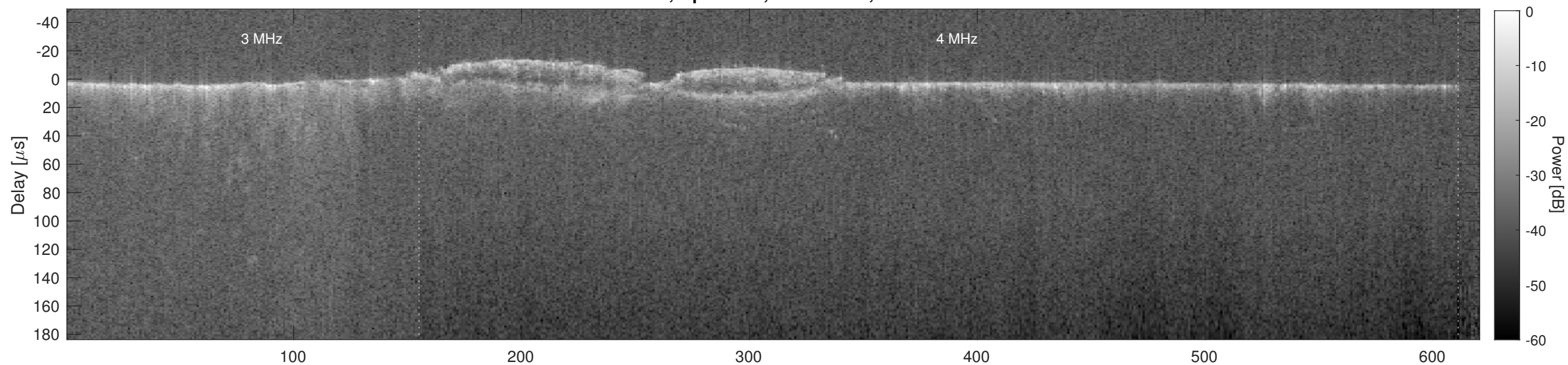
Orbit 7511, Cluttergram
