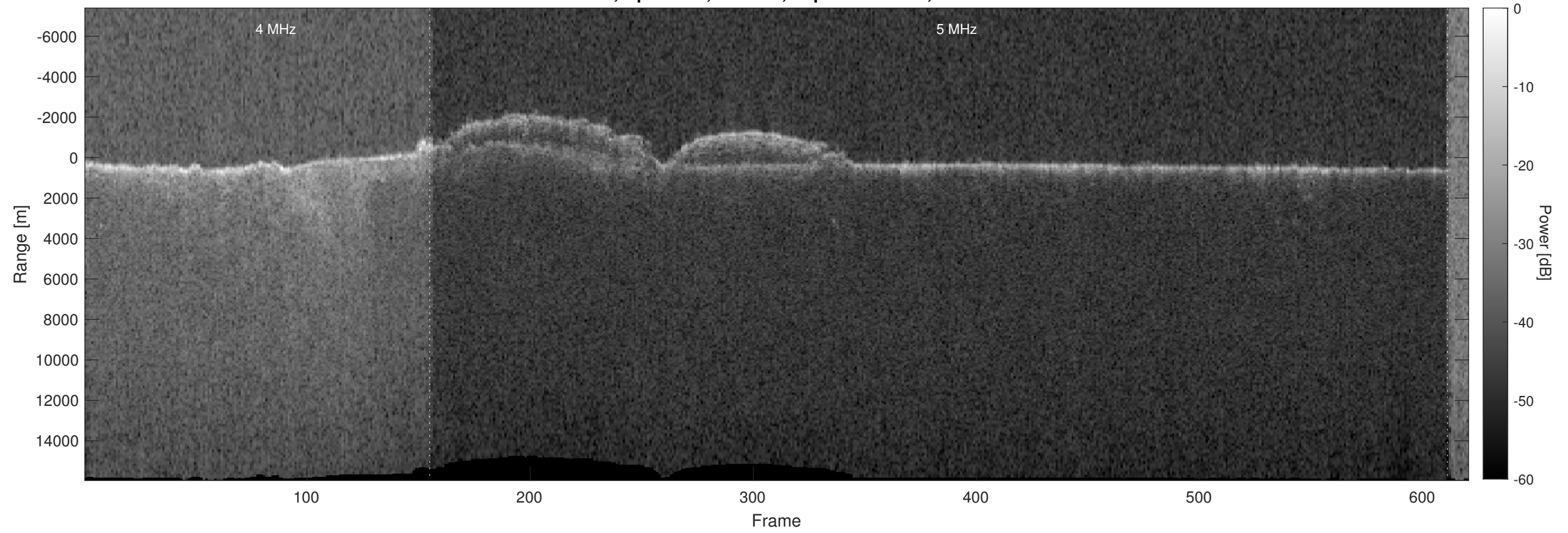
Orbit 7511, Optimized, Window, Depth-Corrected, Channel 2
