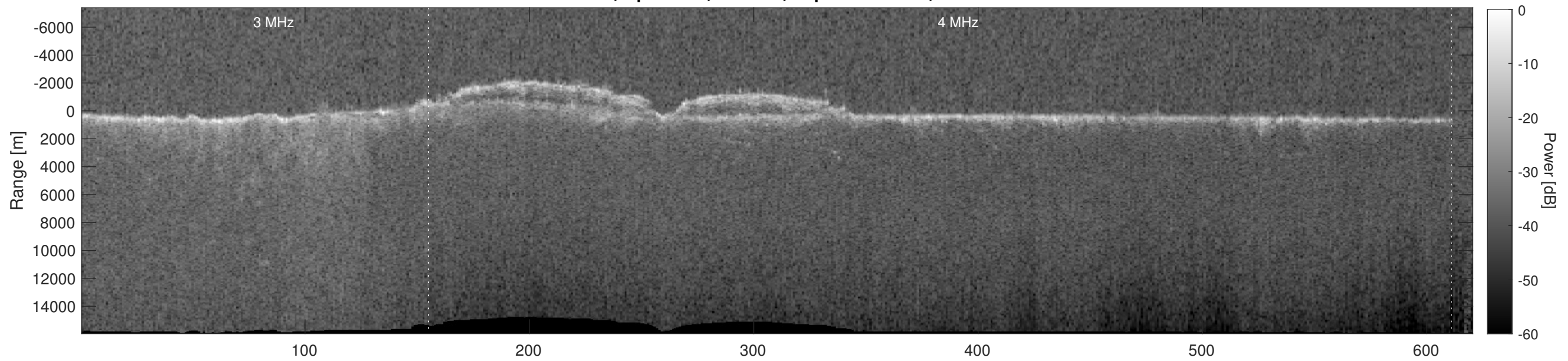
Orbit 7511, Depth-Corrected Cluttergram
