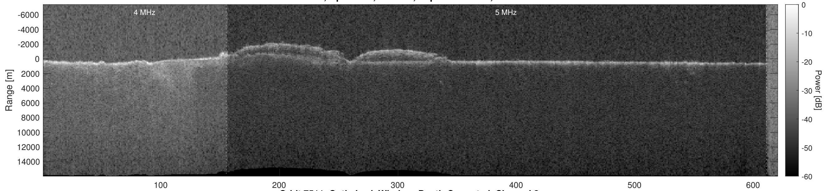
Orbit 7511, Optimized, Window, Depth-Corrected, Channel 2
