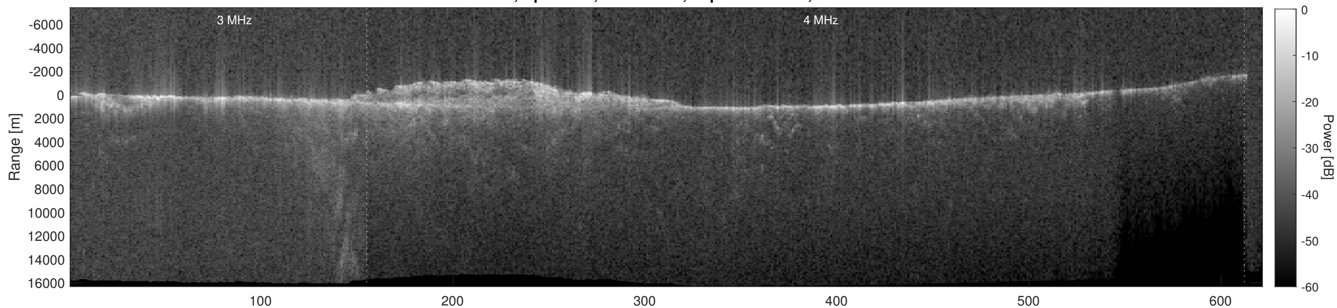
Orbit 7512, Depth-Corrected Cluttergram
