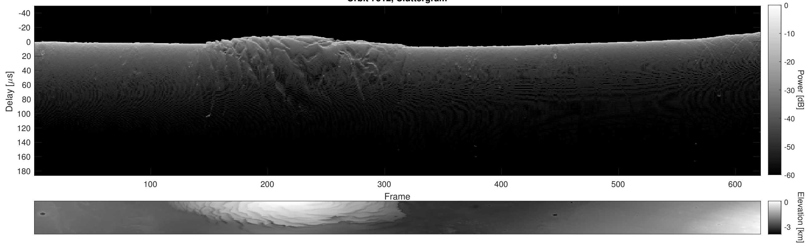
Orbit 7512, Cluttergram
