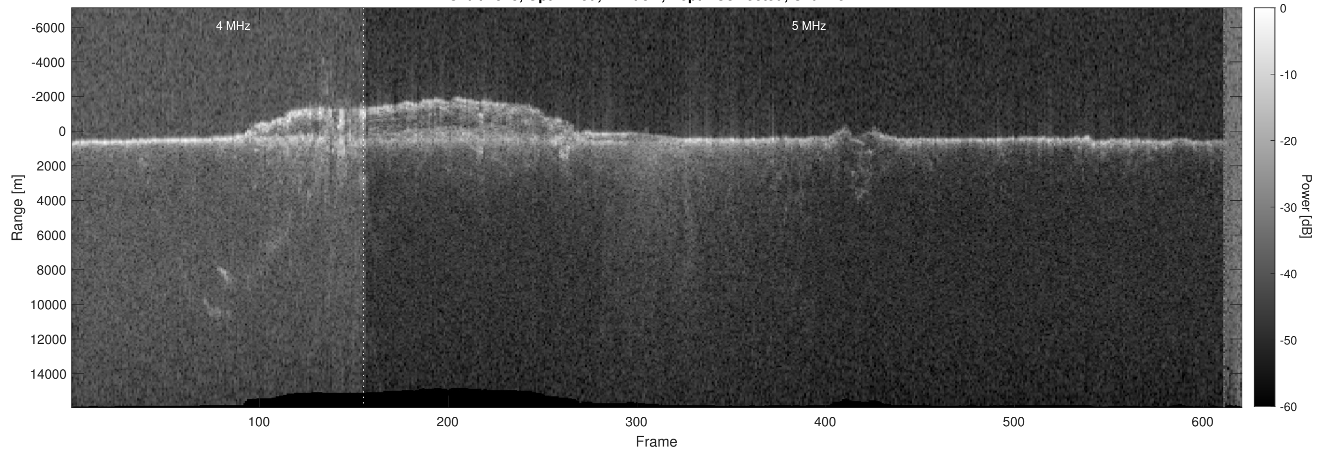
Orbit 7513, Optimized, Window, Depth-Corrected, Channel 2
