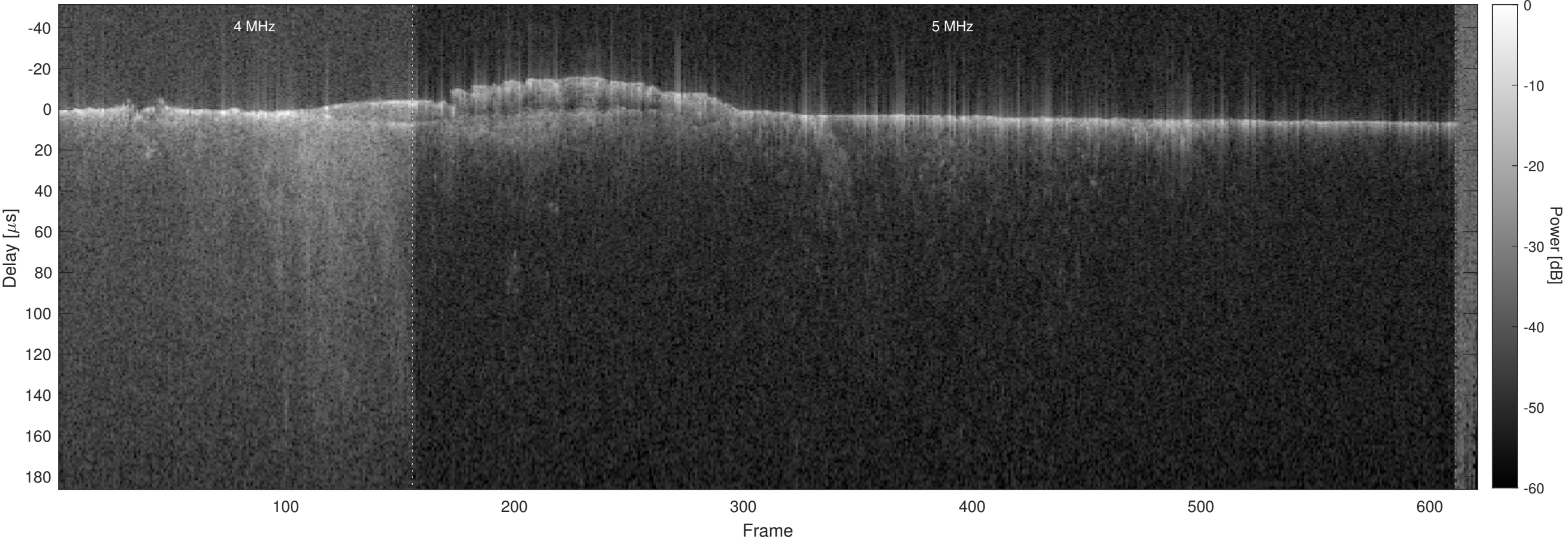
Orbit 7515, Optimized, No Window, Channel 2
