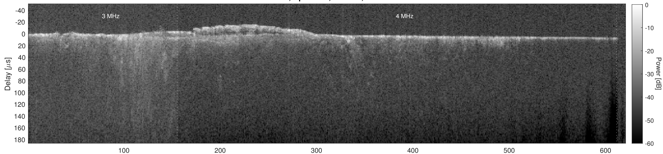
Orbit 7515, Cluttergram
