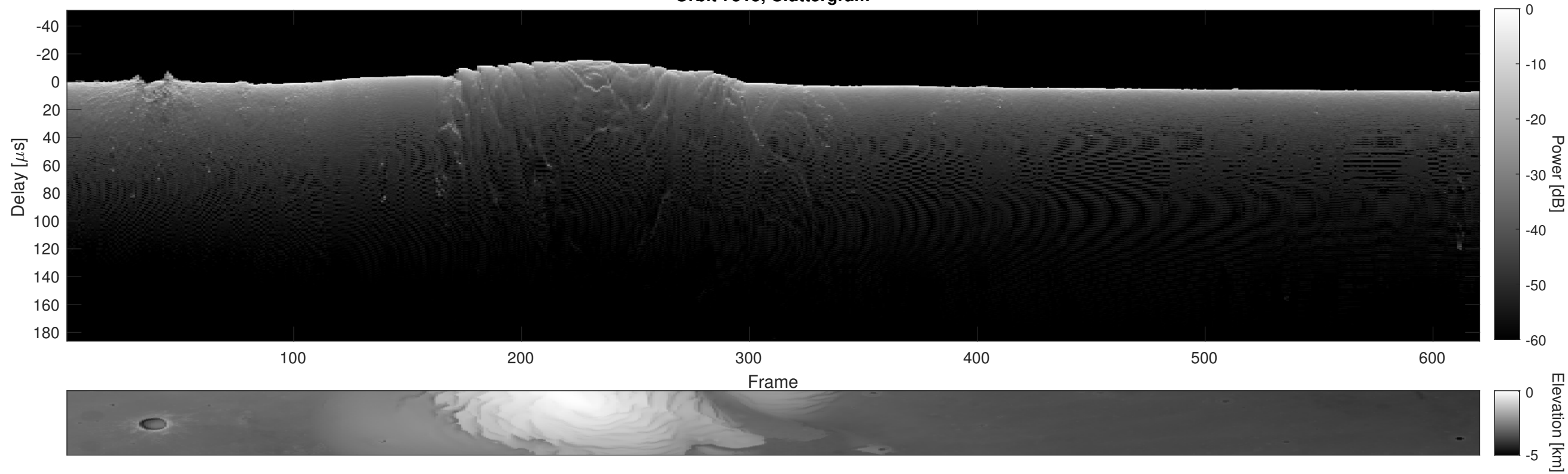
Orbit 7515, Cluttergram
