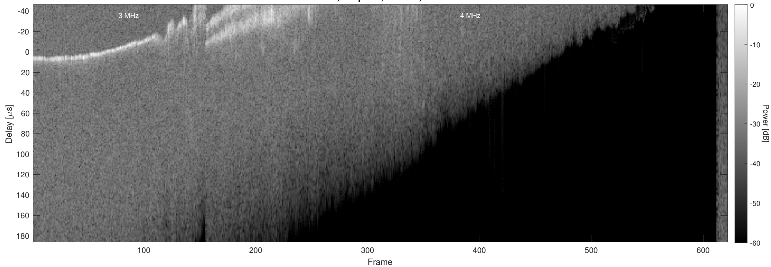
Orbit 7516, Chapman, Window, Channel 2
