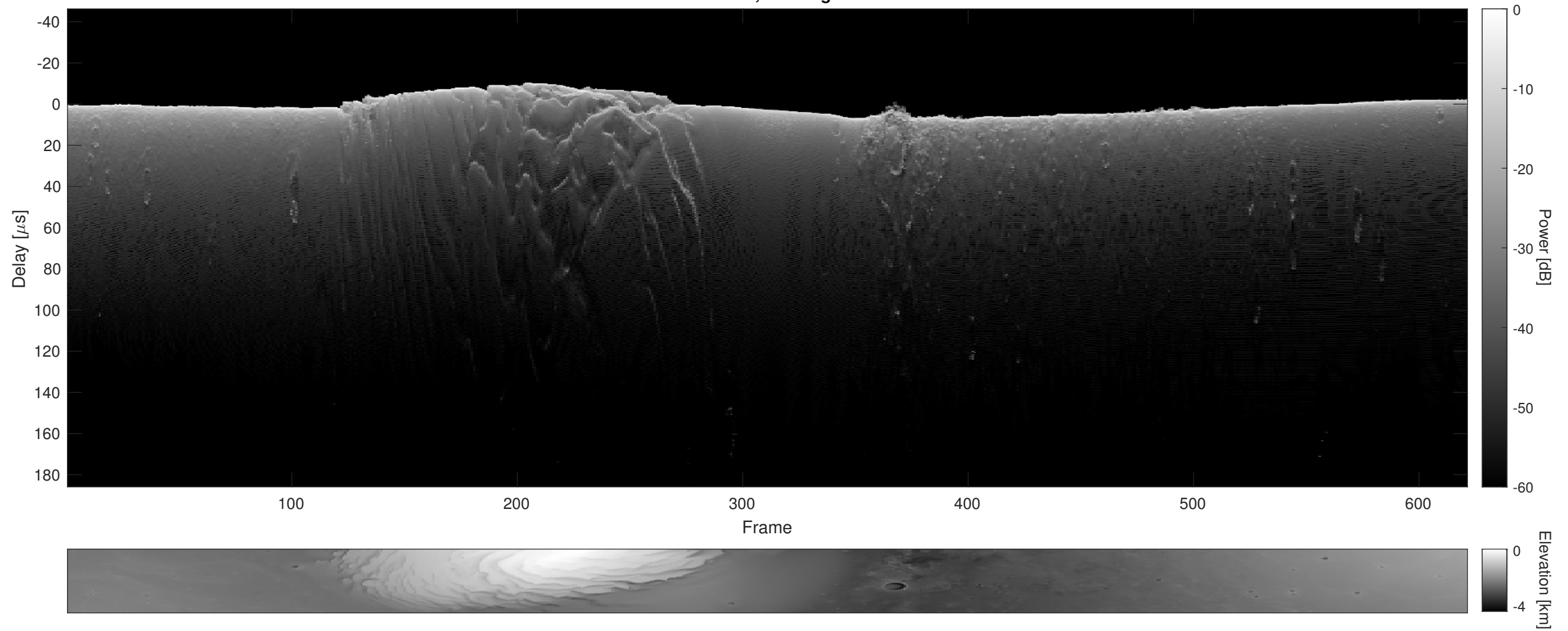
Orbit 7516, Cluttergram
