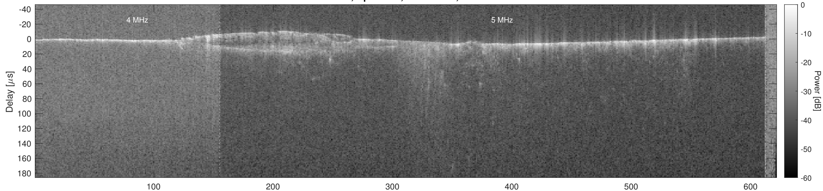
Orbit 7516, Optimized, No Window, Channel 2
