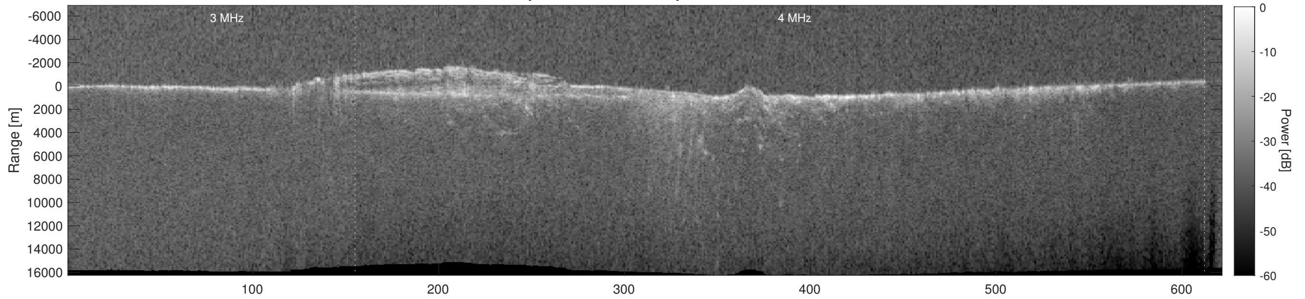
Orbit 7516, Depth-Corrected Cluttergram
