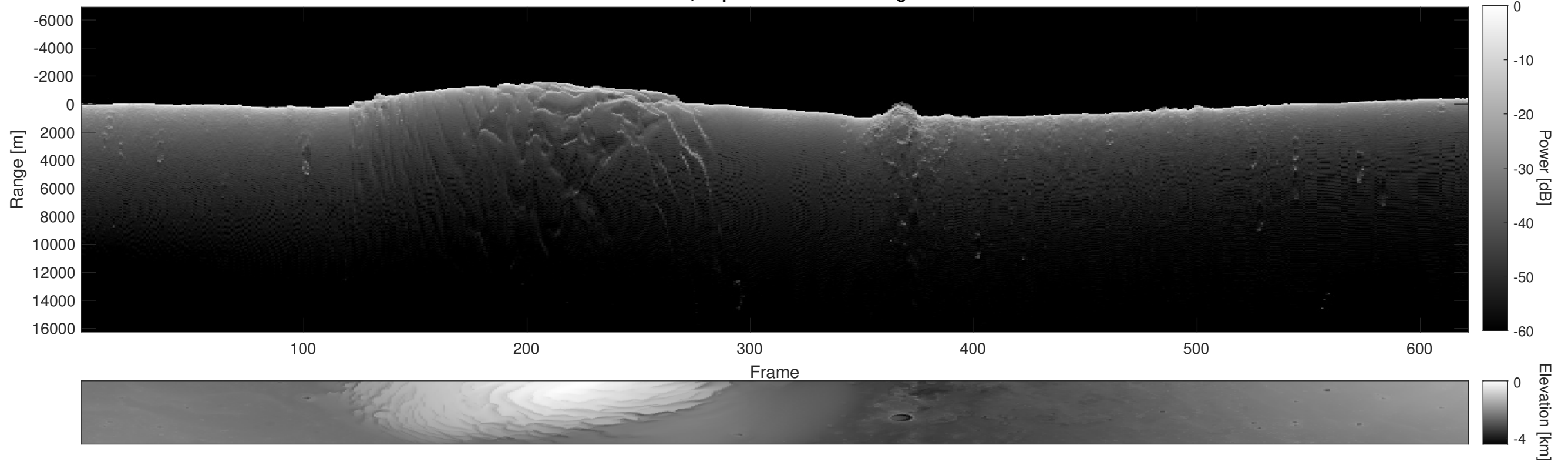
Orbit 7516, Depth-Corrected Cluttergram
