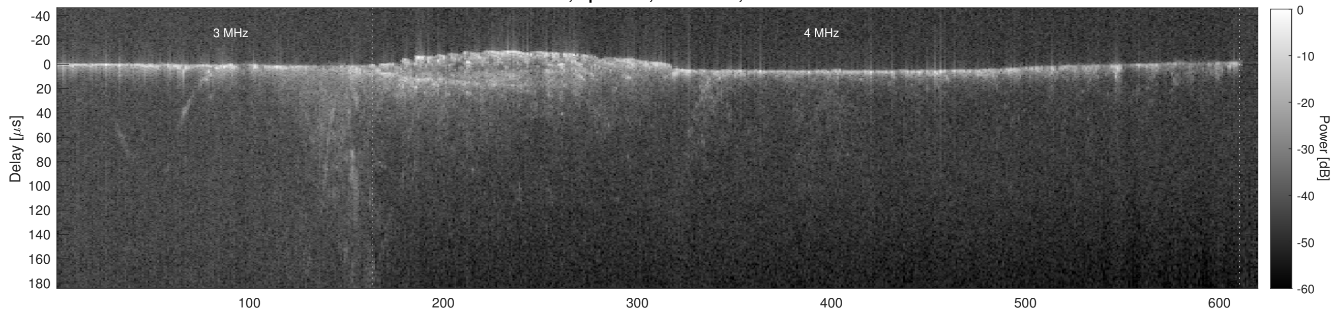
Orbit 7519, Cluttergram
