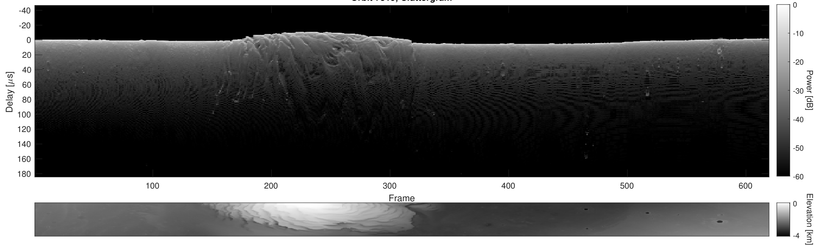
Orbit 7519, Cluttergram
