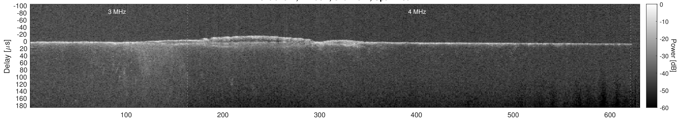
Orbit 7522, Cluttergram
