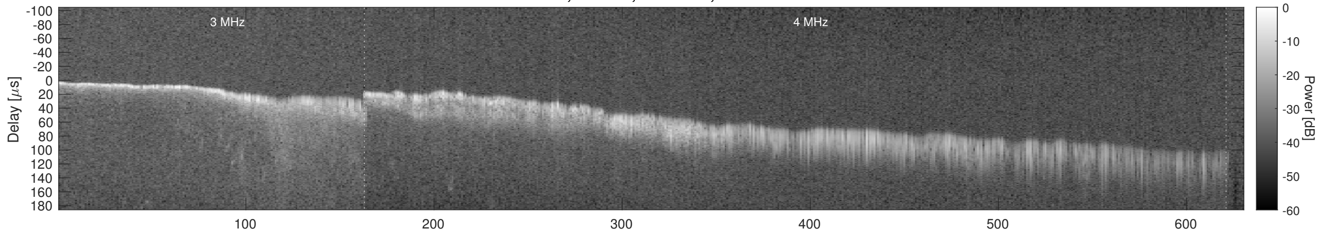
Orbit 7522, Window, Channel 2, Chapman
