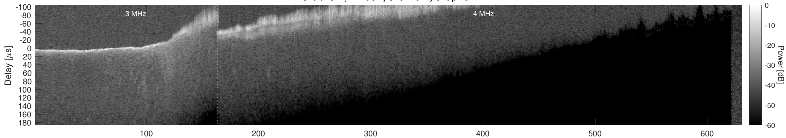
Orbit 7522, Window, Channel 2, Optimized
