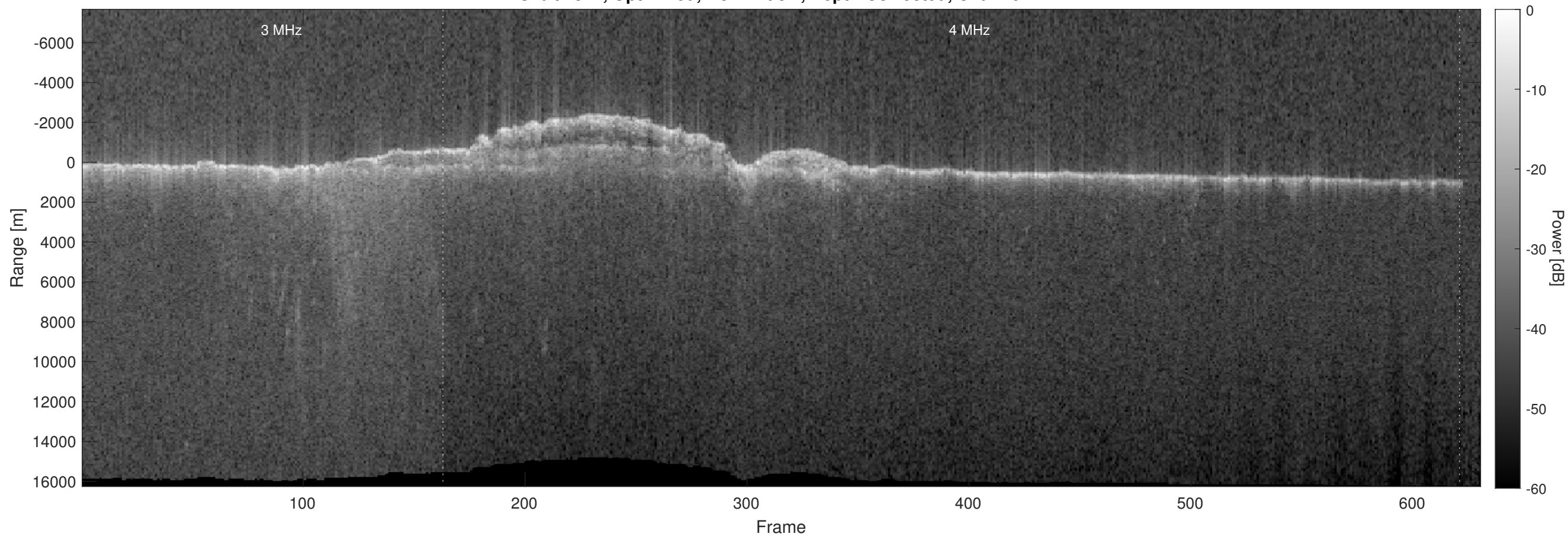
Orbit 7522, Optimized, No Window, Depth-Corrected, Channel 2
