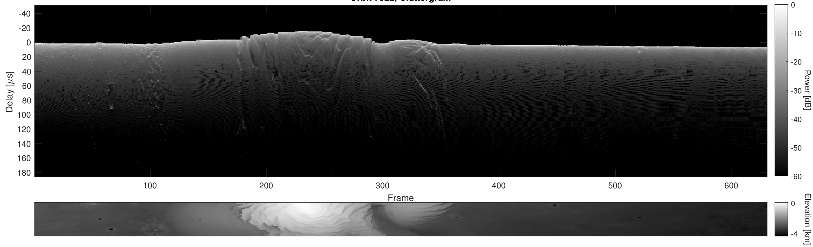
Orbit 7522, Cluttergram
