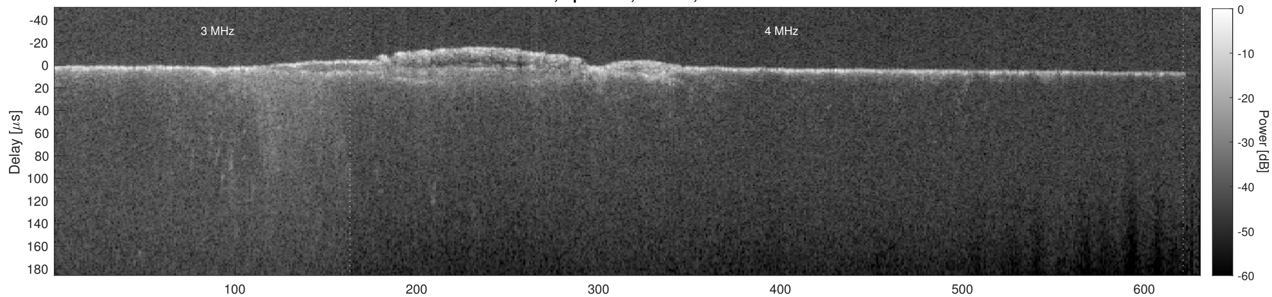
Orbit 7522, Cluttergram
