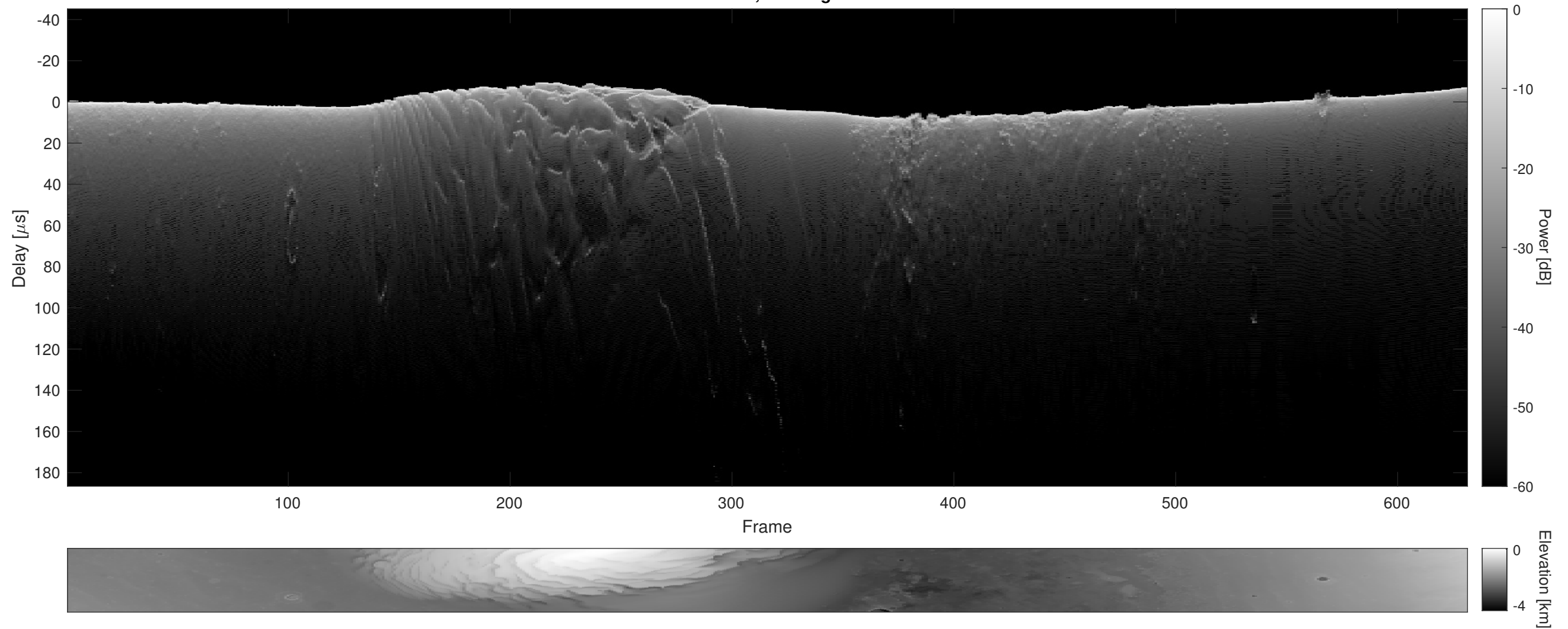
Orbit 7523, Cluttergram
