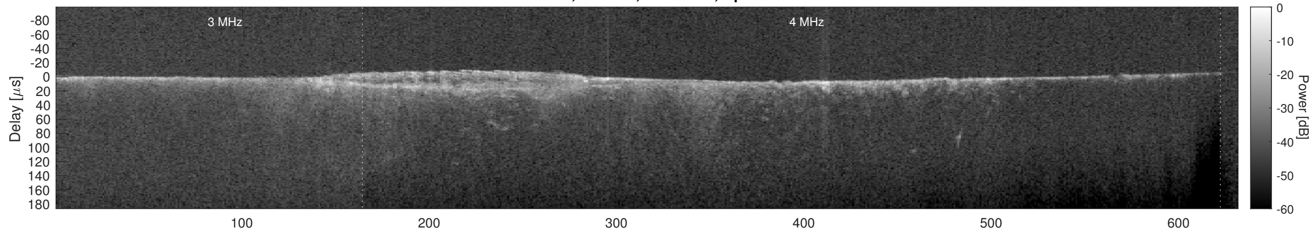
Orbit 7523, Cluttergram
