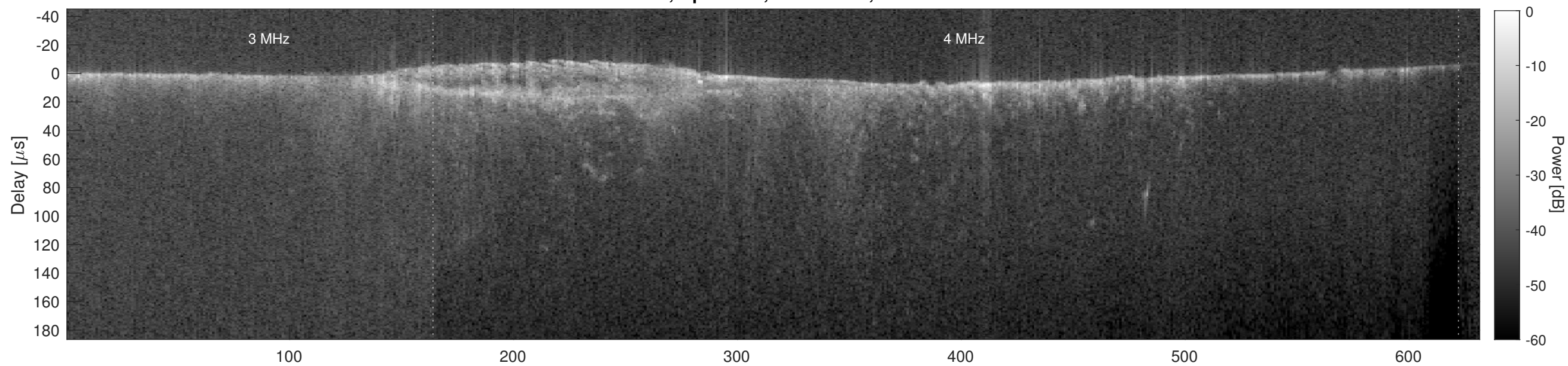
Orbit 7523, Cluttergram
