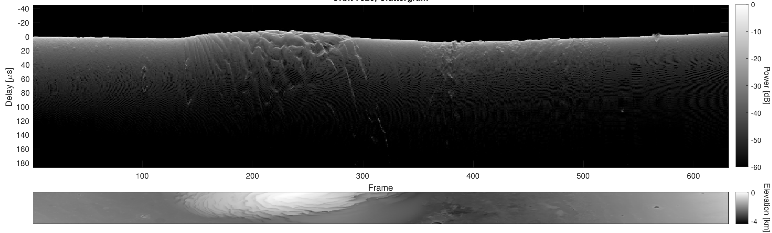
Orbit 7523, Cluttergram
