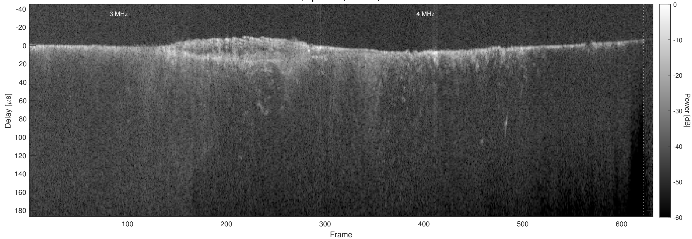
Orbit 7523, Optimized, Window, Channel 2
