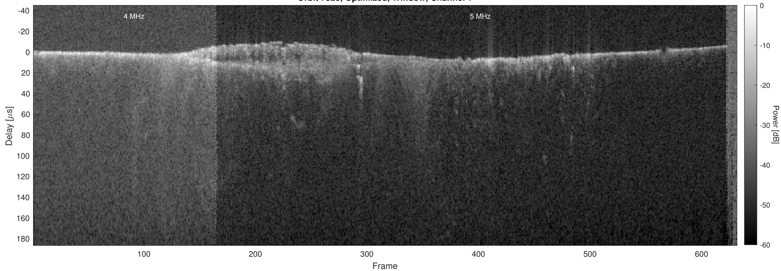
Orbit 7523, Optimized, Window, Channel 2
