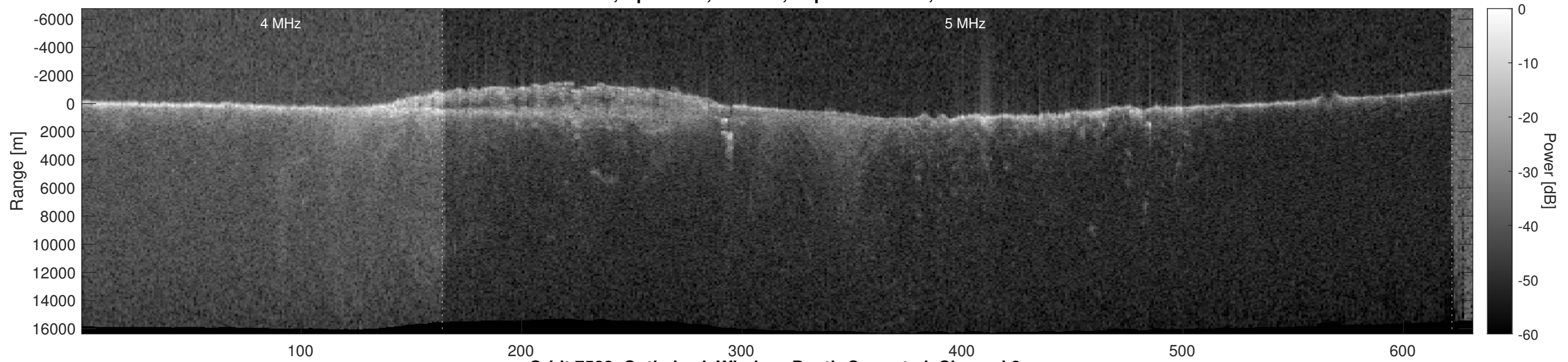
Orbit 7523, Optimized, Window, Depth-Corrected, Channel 2
