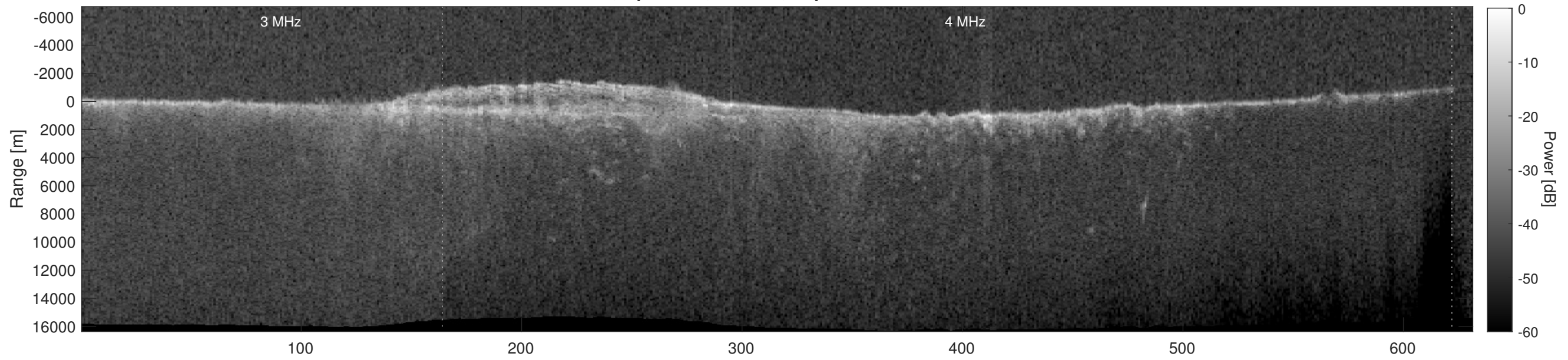
Orbit 7523, Depth-Corrected Cluttergram
