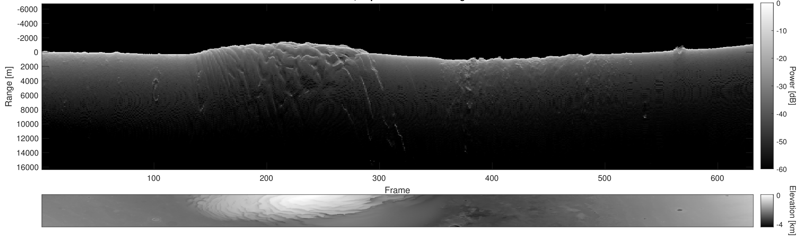
Orbit 7523, Depth-Corrected Cluttergram
