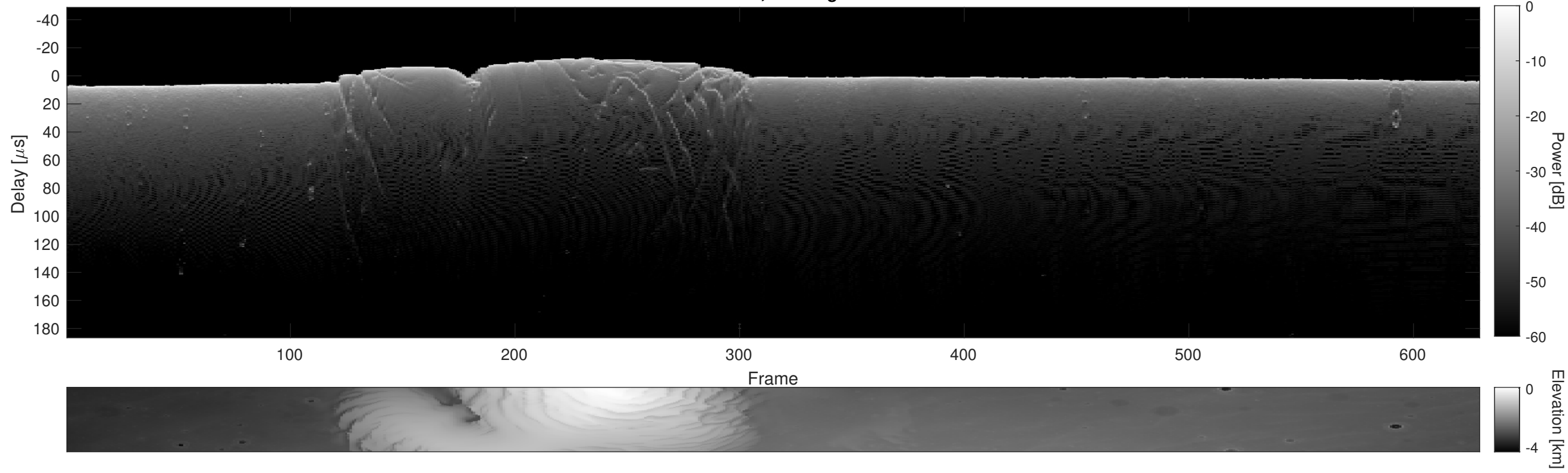
Orbit 7524, Cluttergram
