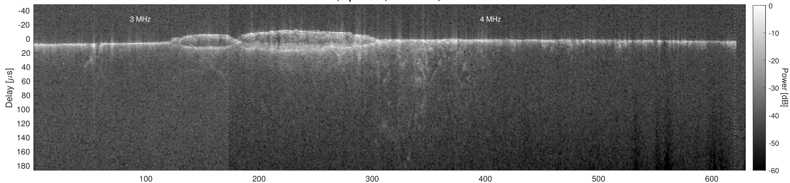
Orbit 7524, Cluttergram
