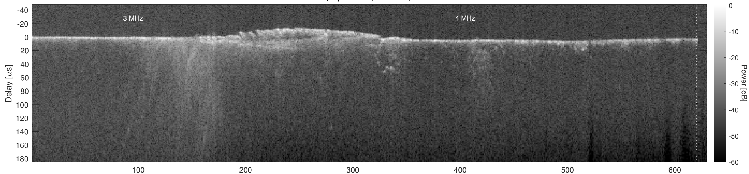
Orbit 7526, Cluttergram
