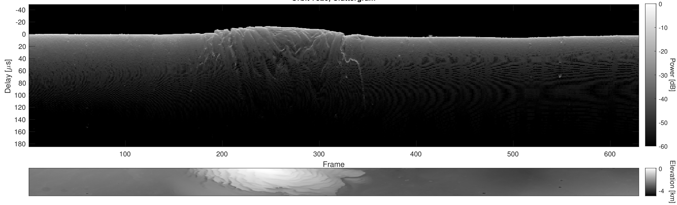
Orbit 7526, Cluttergram
