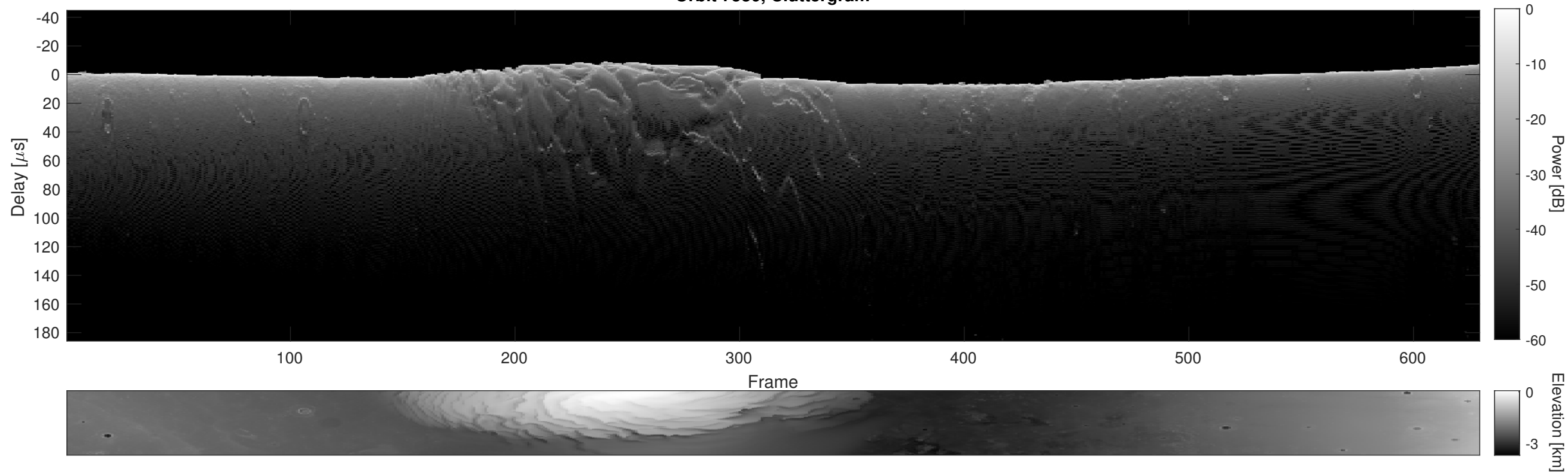
Orbit 7530, Cluttergram
