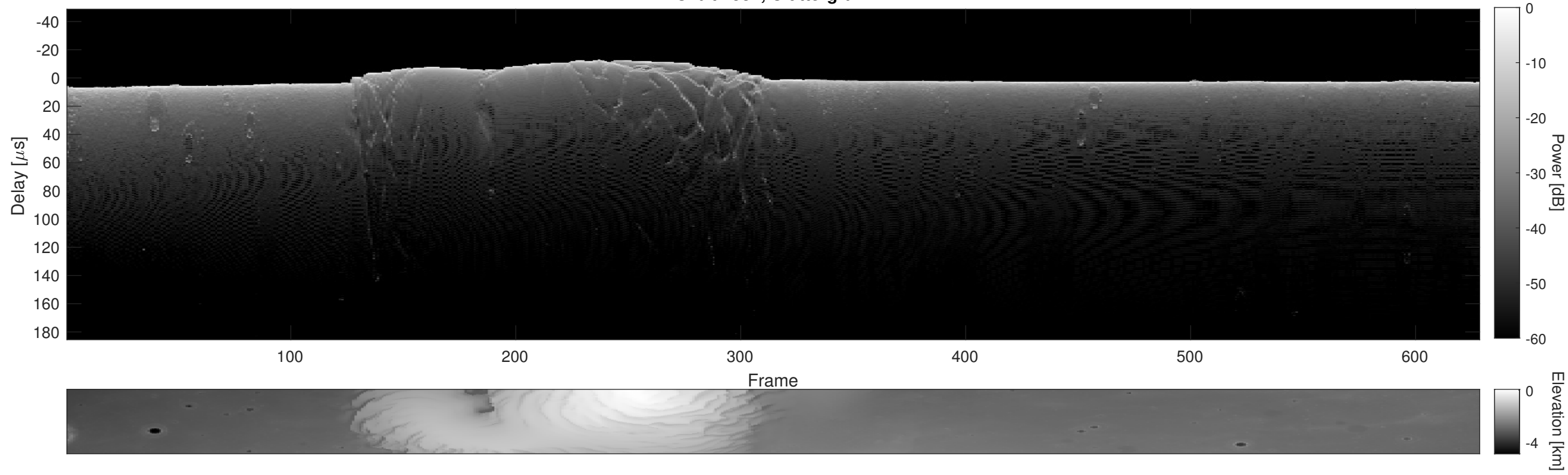
Orbit 7531, Cluttergram
