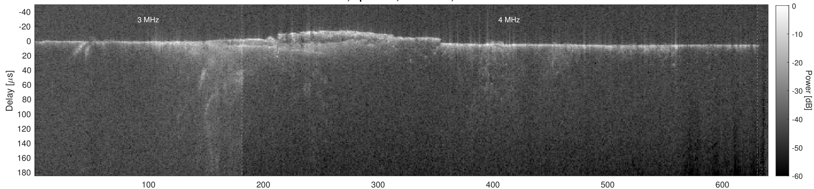
Orbit 7533, Cluttergram
