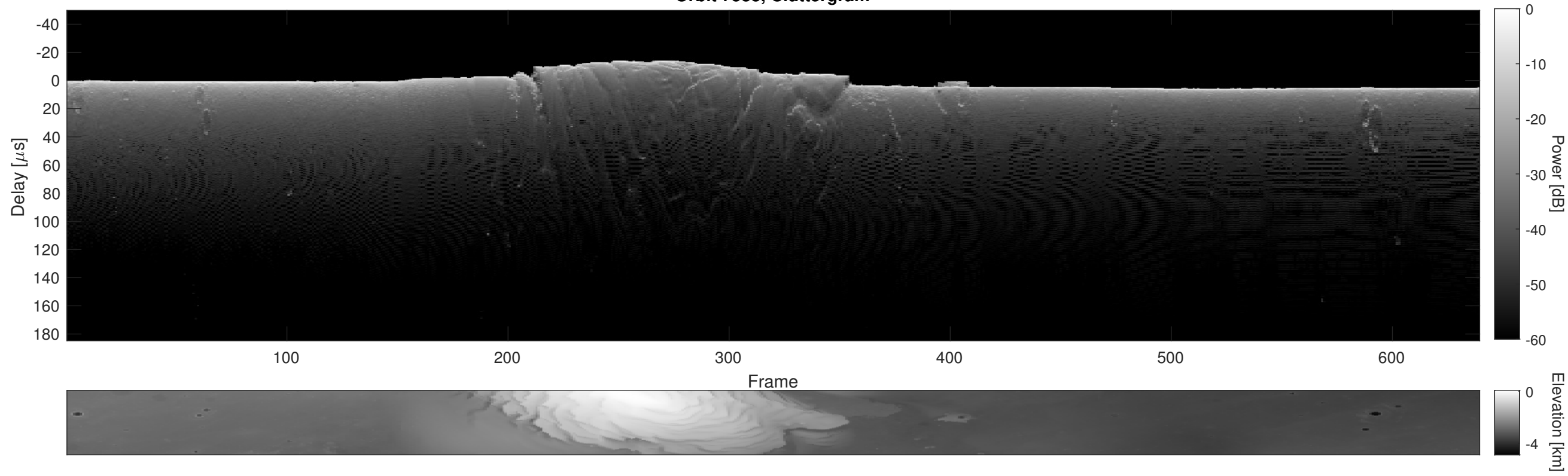
Orbit 7533, Cluttergram
