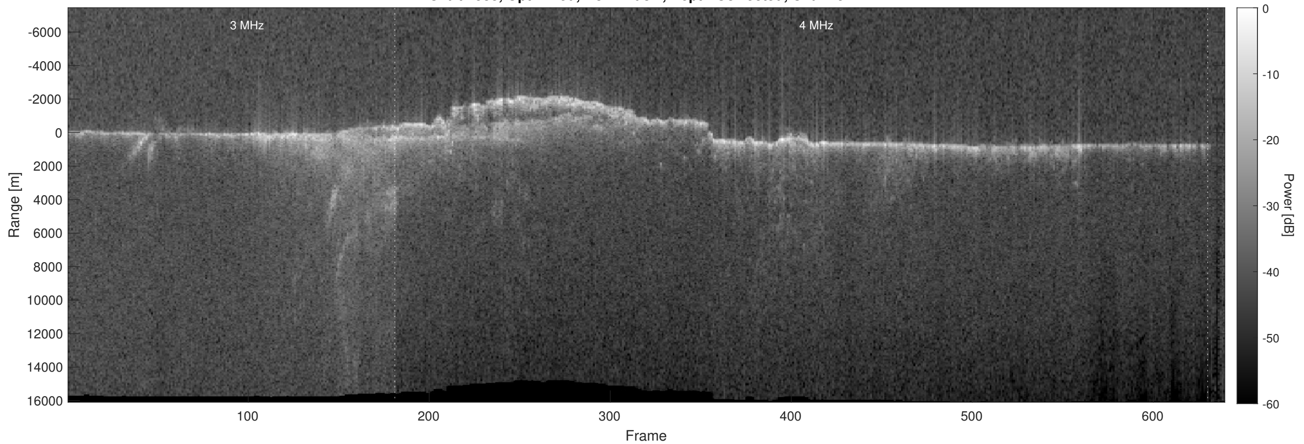
Orbit 7533, Optimized, No Window, Depth-Corrected, Channel 2
