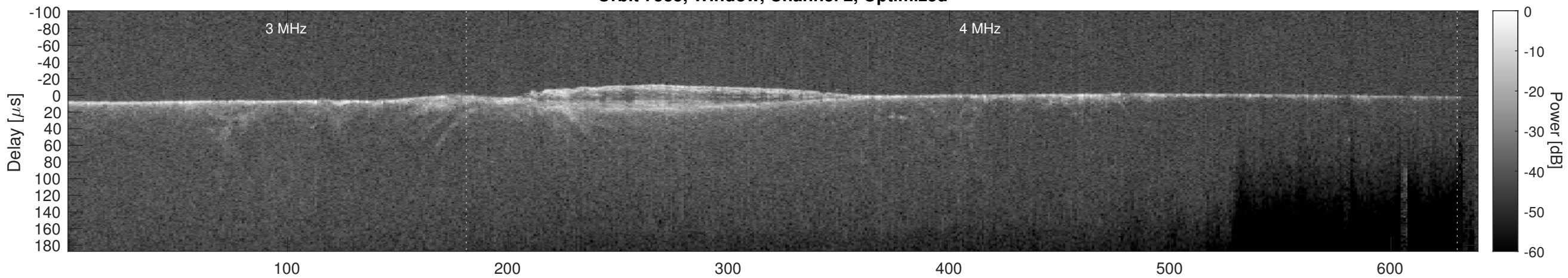
Orbit 7535, Cluttergram
