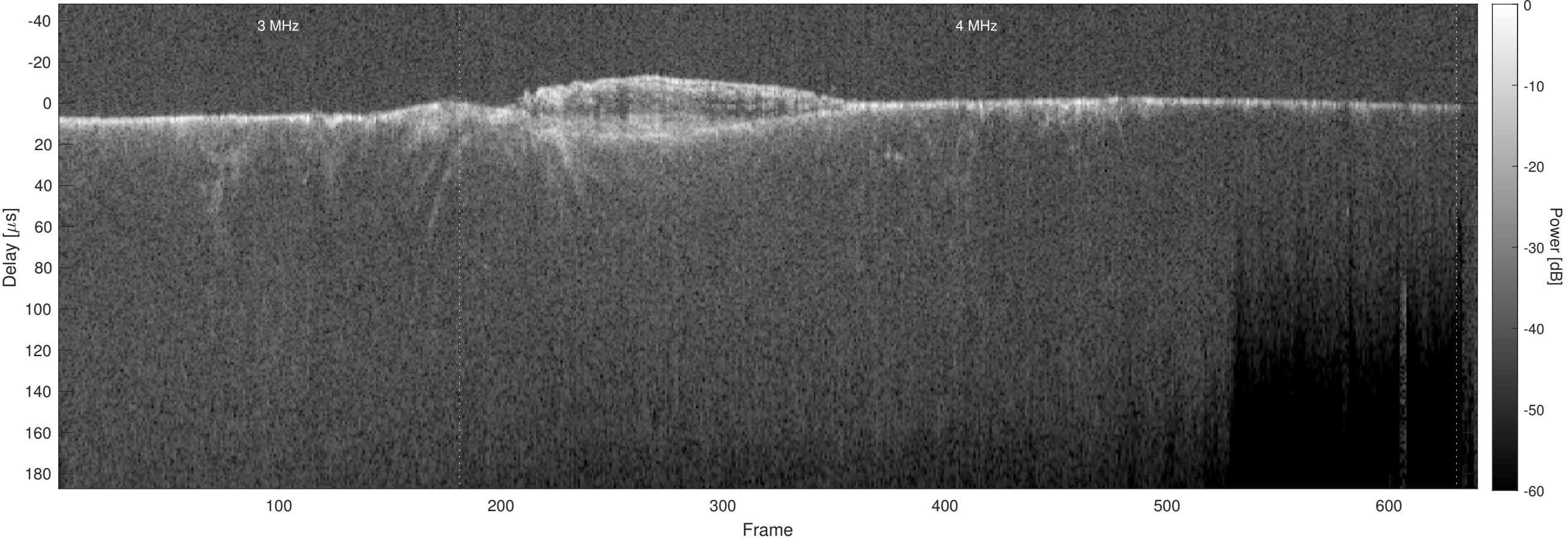
Orbit 7535, Optimized, Window, Channel 2
