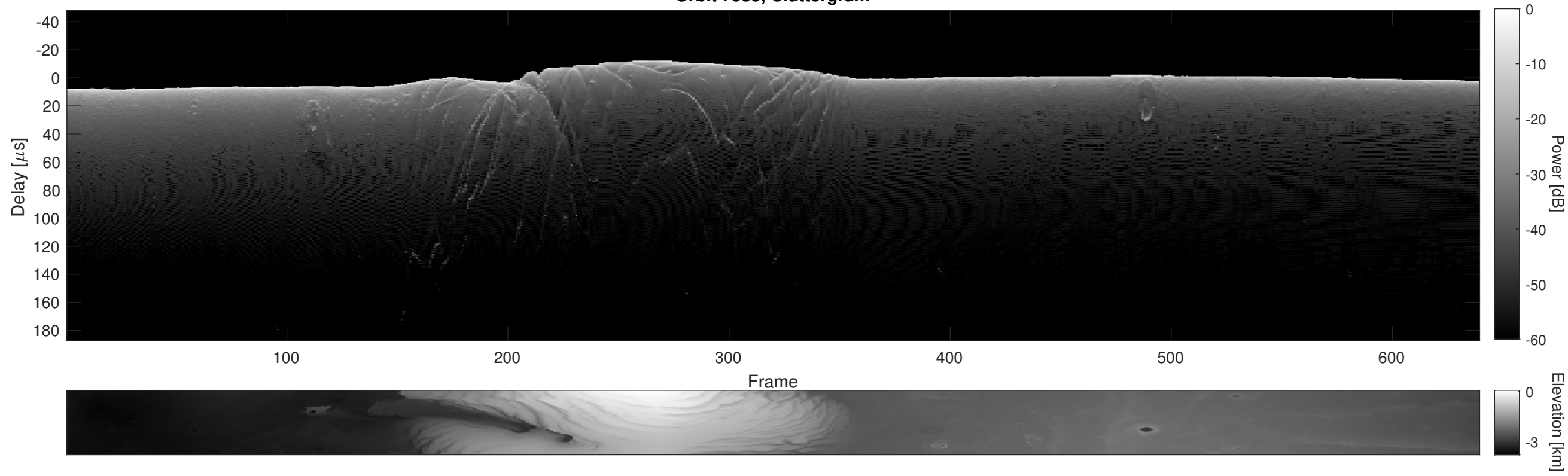
Orbit 7535, Cluttergram
