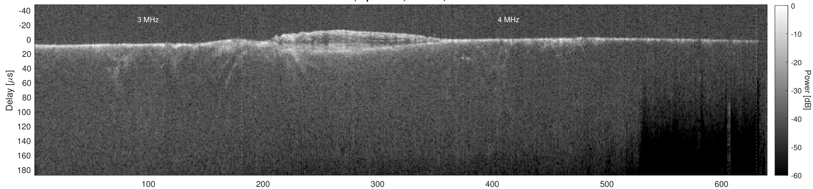
Orbit 7535, Cluttergram
