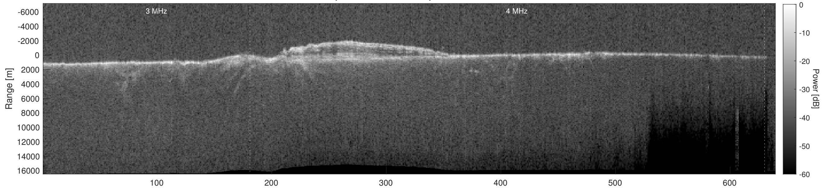
Orbit 7535, Depth-Corrected Cluttergram
