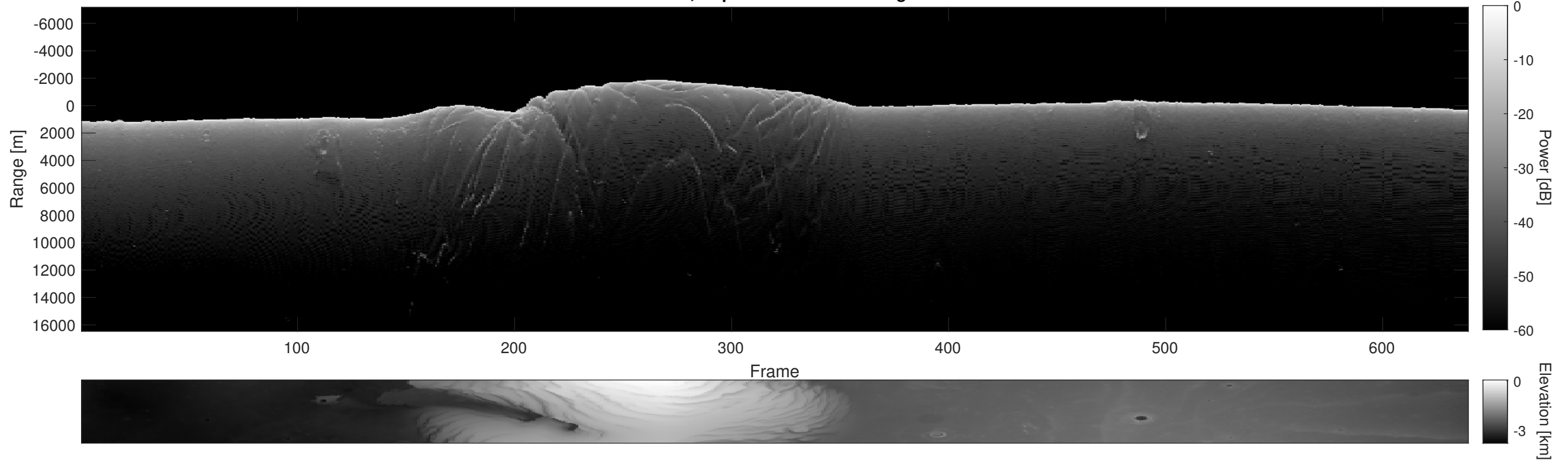
Orbit 7535, Depth-Corrected Cluttergram
