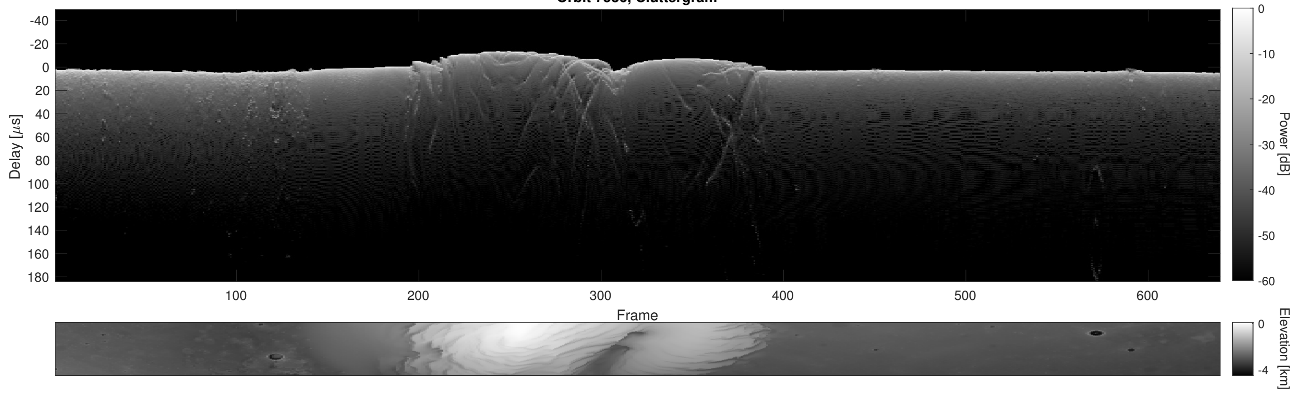
Orbit 7536, Cluttergram
