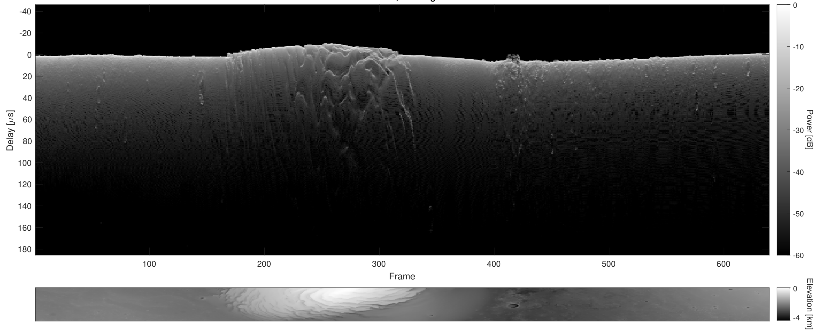
Orbit 7541, Cluttergram
