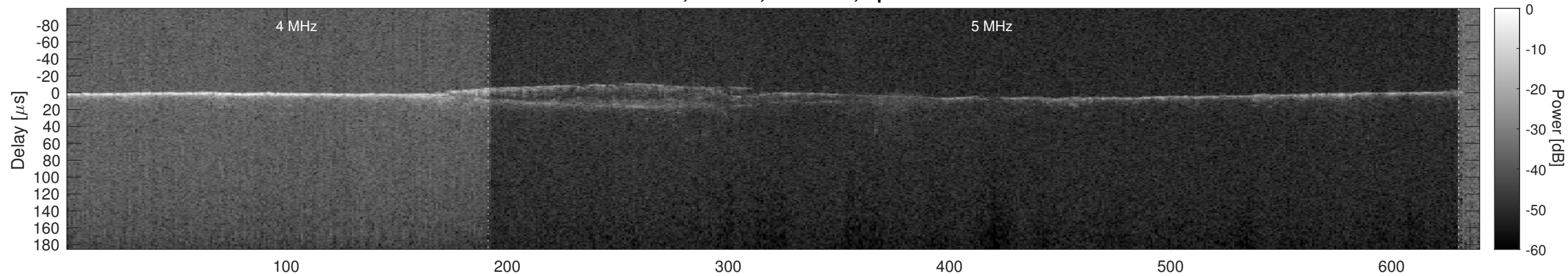
Orbit 7541, Cluttergram
