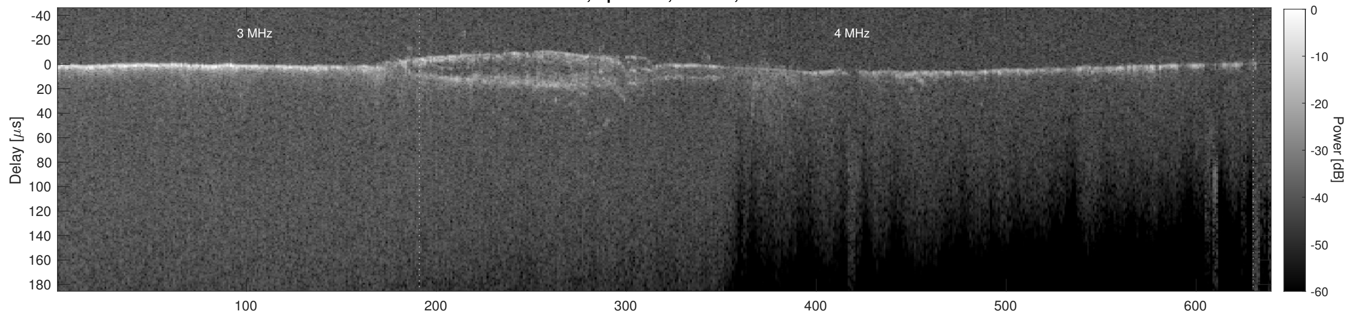
Orbit 7541, Cluttergram
