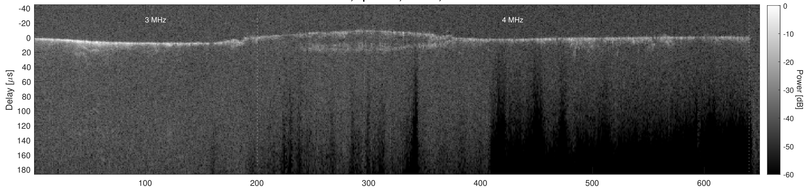
Orbit 7546, Cluttergram
