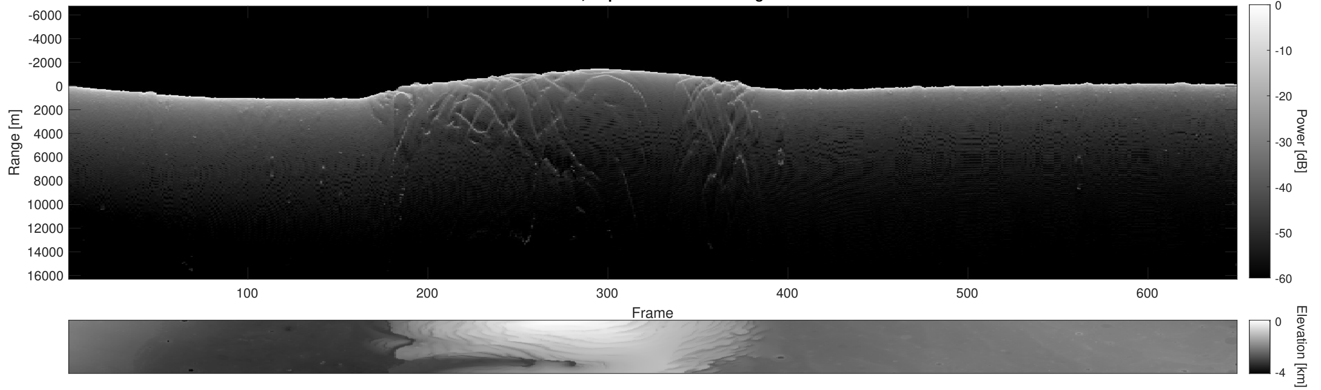
Orbit 7546, Depth-Corrected Cluttergram
