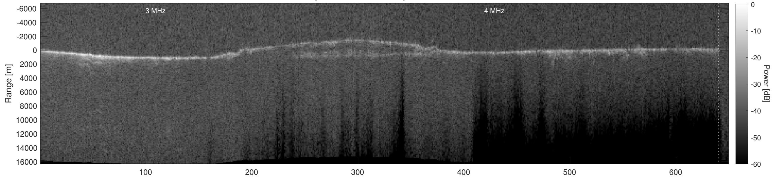
Orbit 7546, Depth-Corrected Cluttergram
