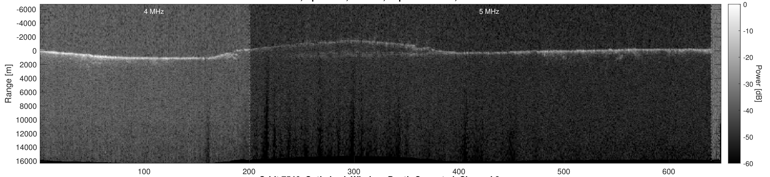
Orbit 7546, Optimized, Window, Depth-Corrected, Channel 2
