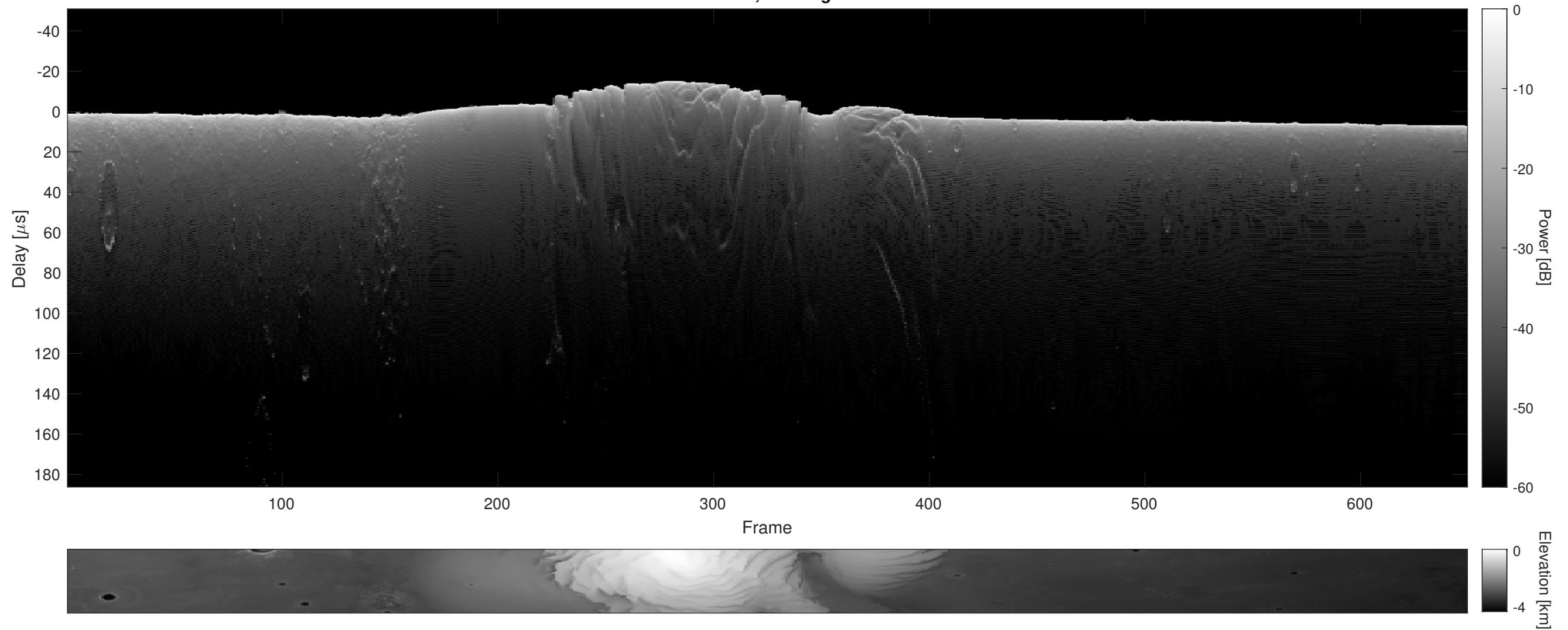
Orbit 7547, Cluttergram
