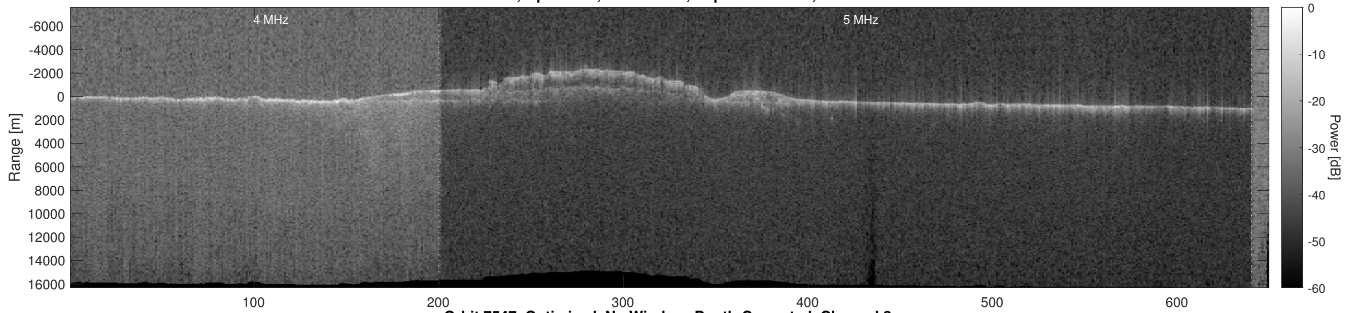
Orbit 7547, Optimized, No Window, Depth-Corrected, Channel 2
