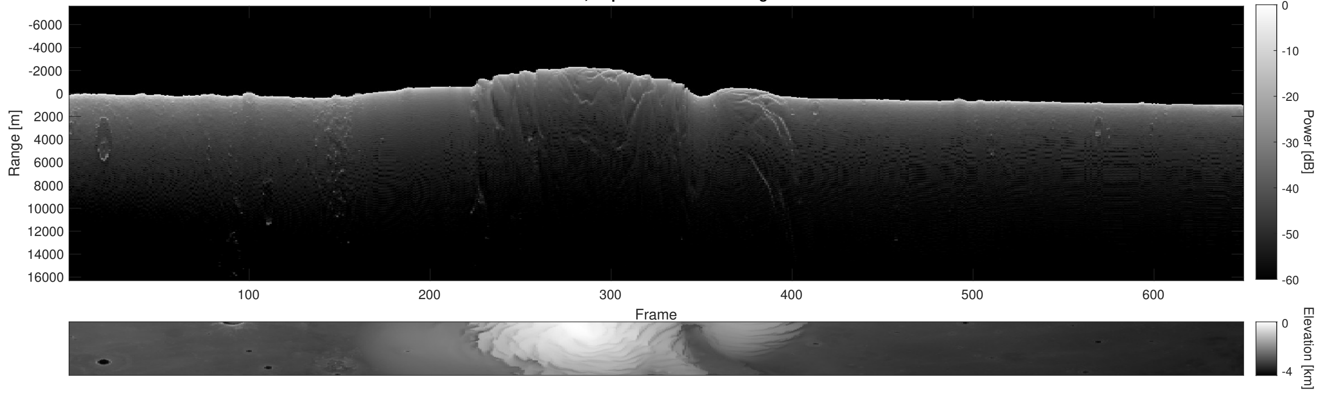
Orbit 7547, Depth-Corrected Cluttergram
