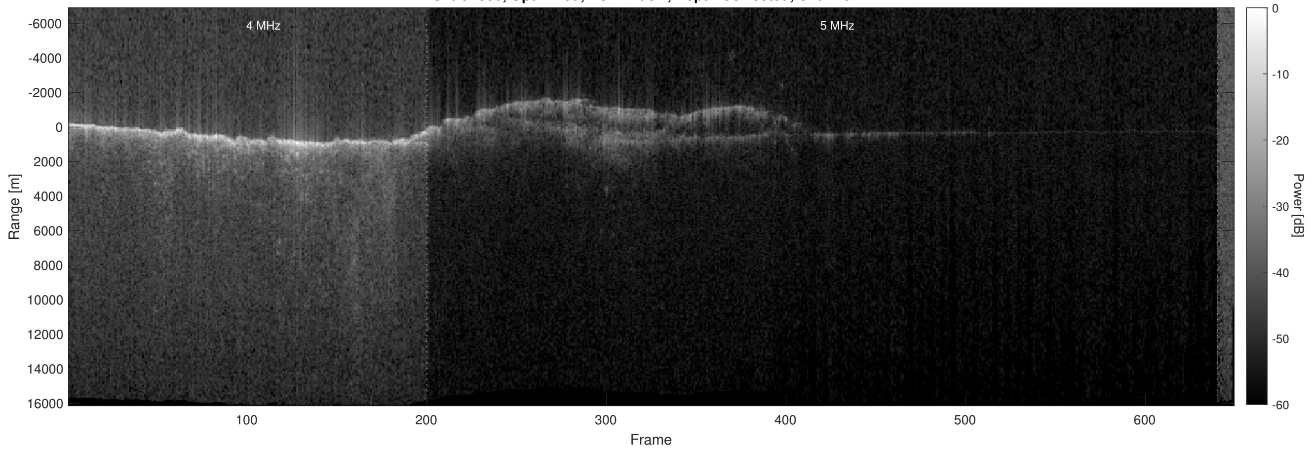
Orbit 7550, Optimized, No Window, Depth-Corrected, Channel 2
