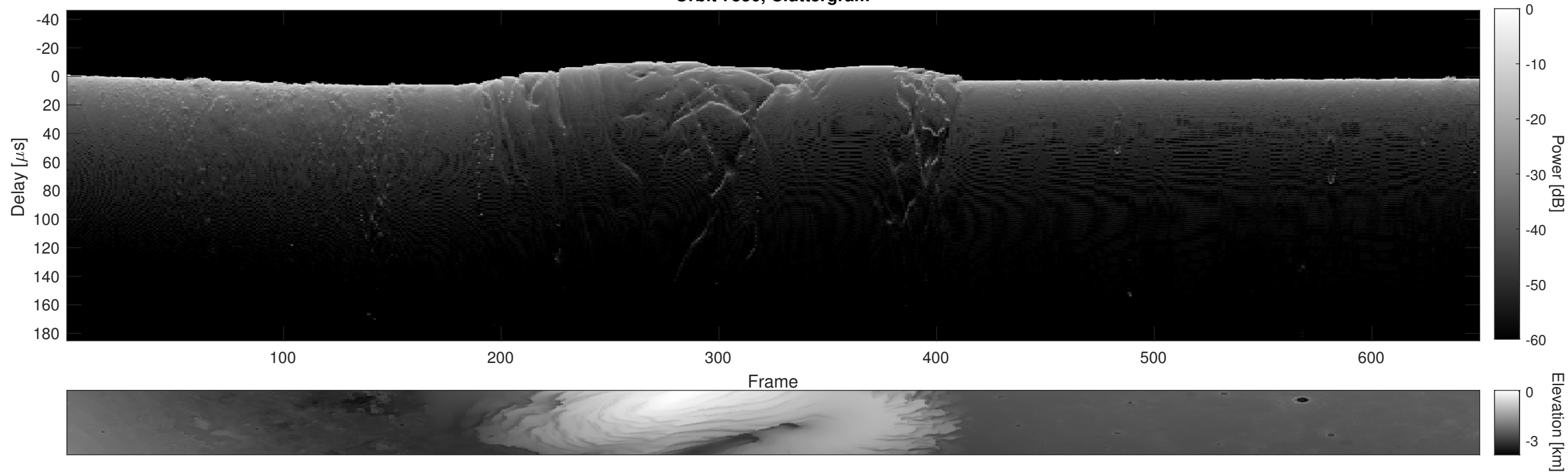
Orbit 7550, Cluttergram
