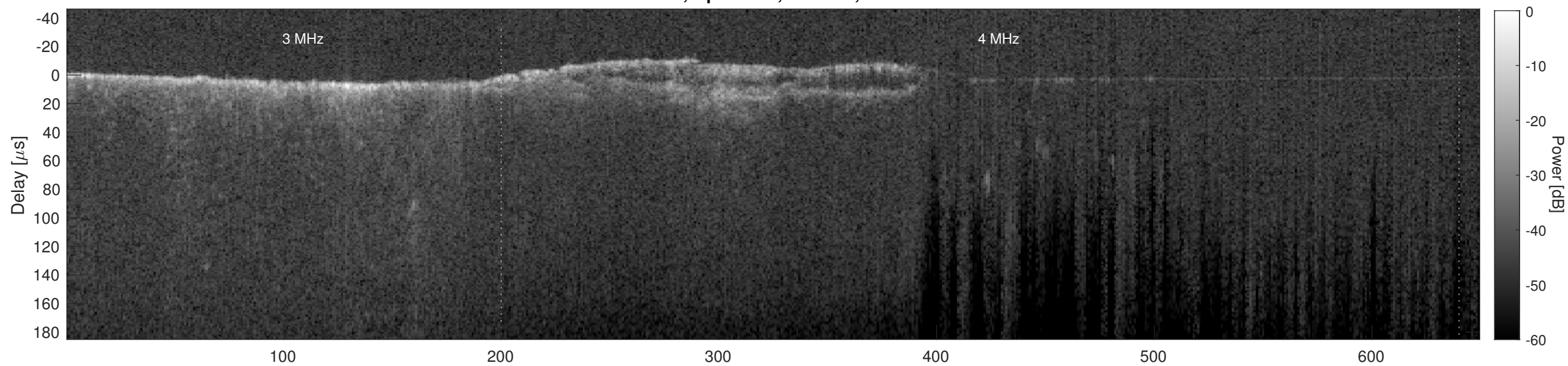
Orbit 7550, Cluttergram
