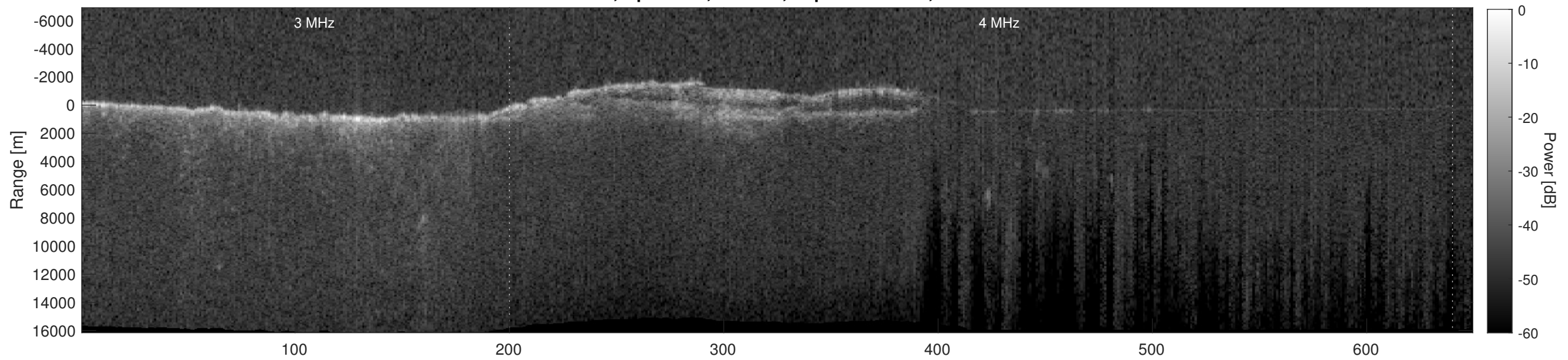
Orbit 7550, Depth-Corrected Cluttergram
