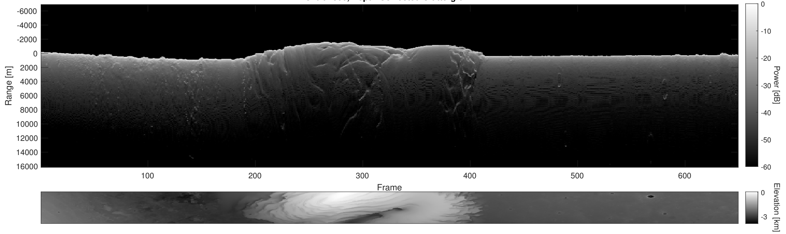
Orbit 7550, Depth-Corrected Cluttergram
