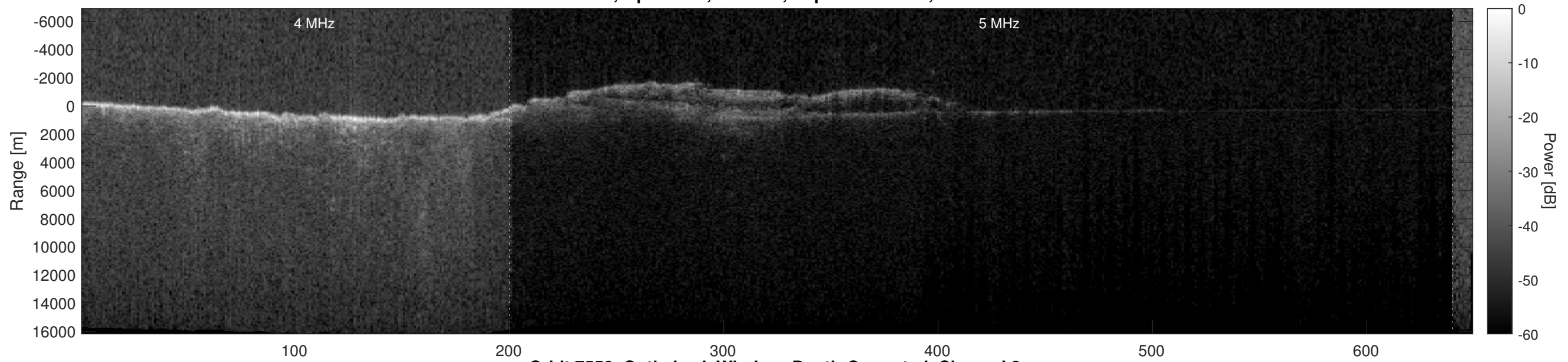
Orbit 7550, Optimized, Window, Depth-Corrected, Channel 2
