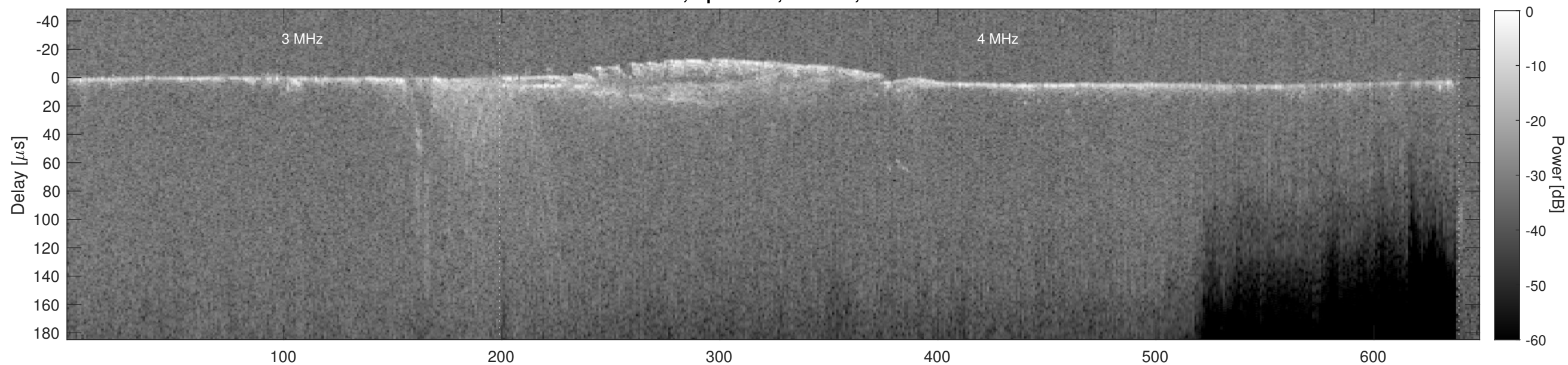
Orbit 7551, Cluttergram
