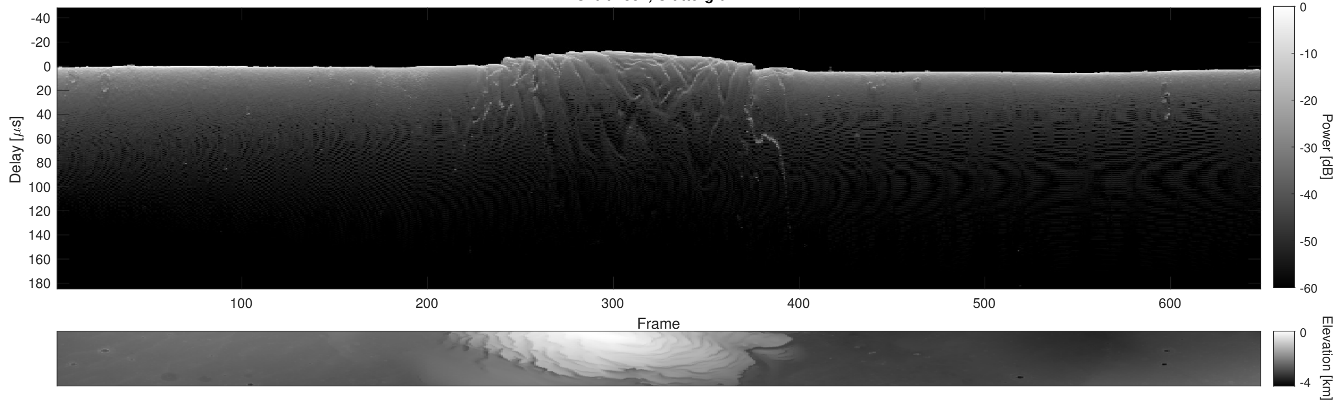
Orbit 7551, Cluttergram
