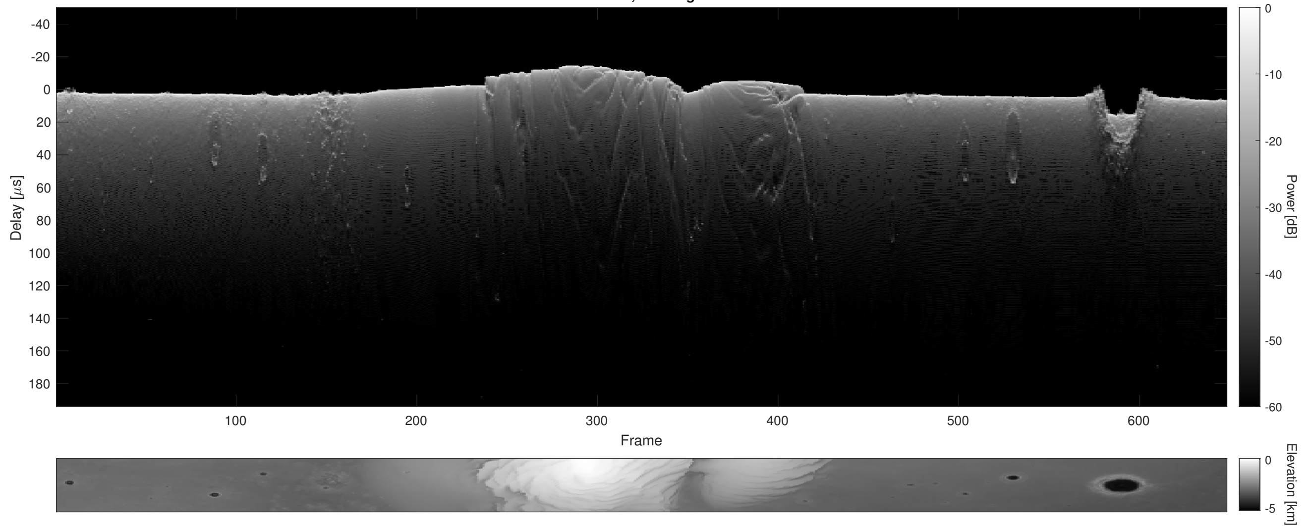
Orbit 7554, Cluttergram
