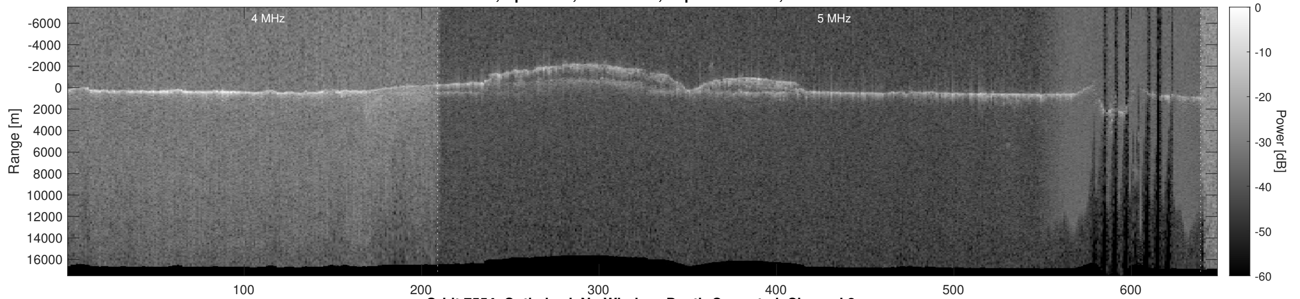
Orbit 7554, Optimized, No Window, Depth-Corrected, Channel 2
