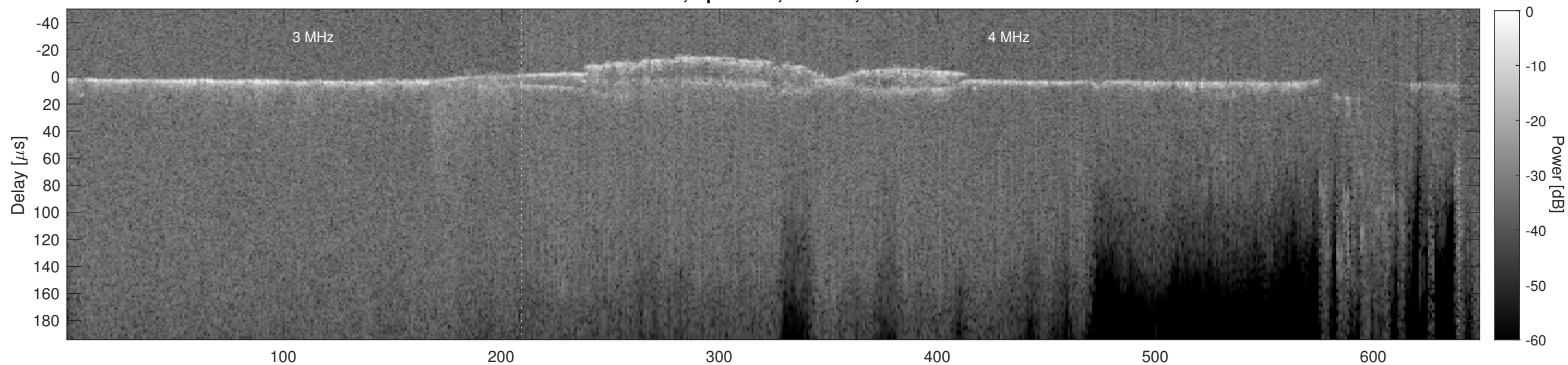
Orbit 7554, Cluttergram
