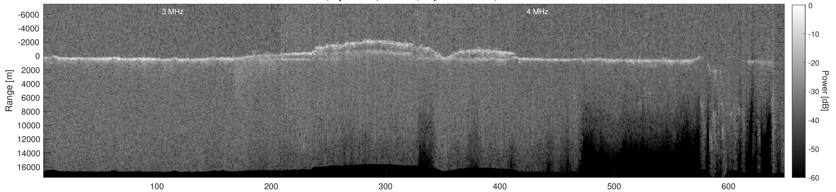
Orbit 7554, Depth-Corrected Cluttergram
