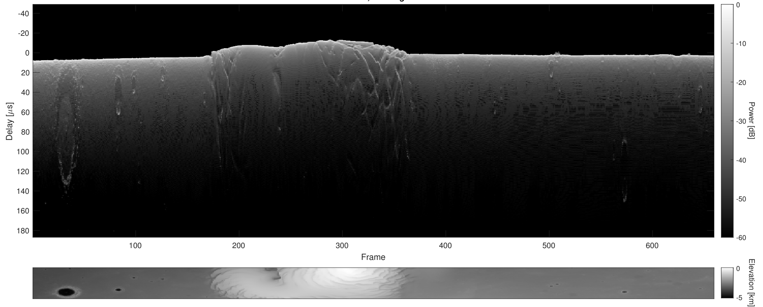
Orbit 7556, Cluttergram
