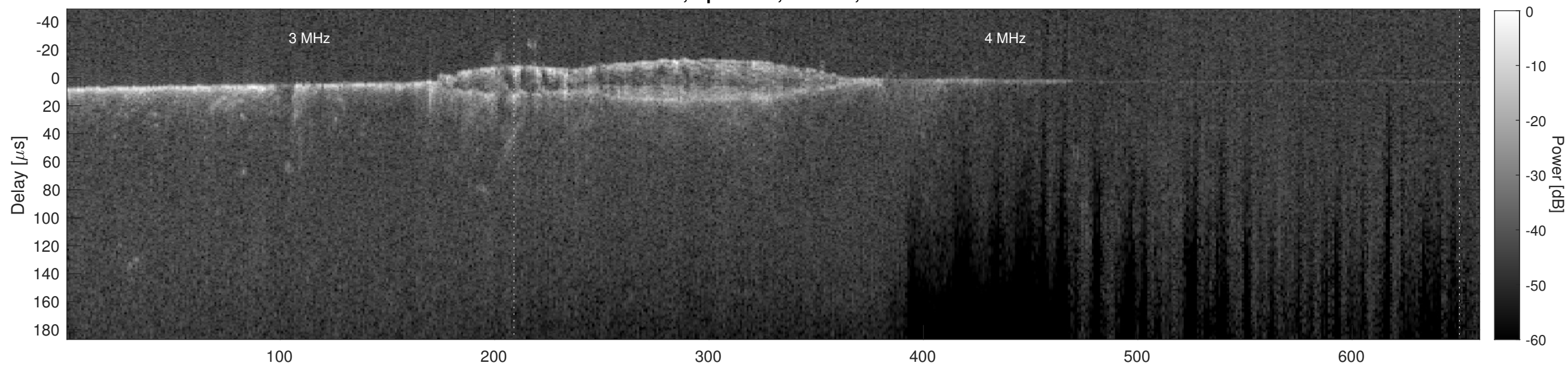
Orbit 7556, Cluttergram
