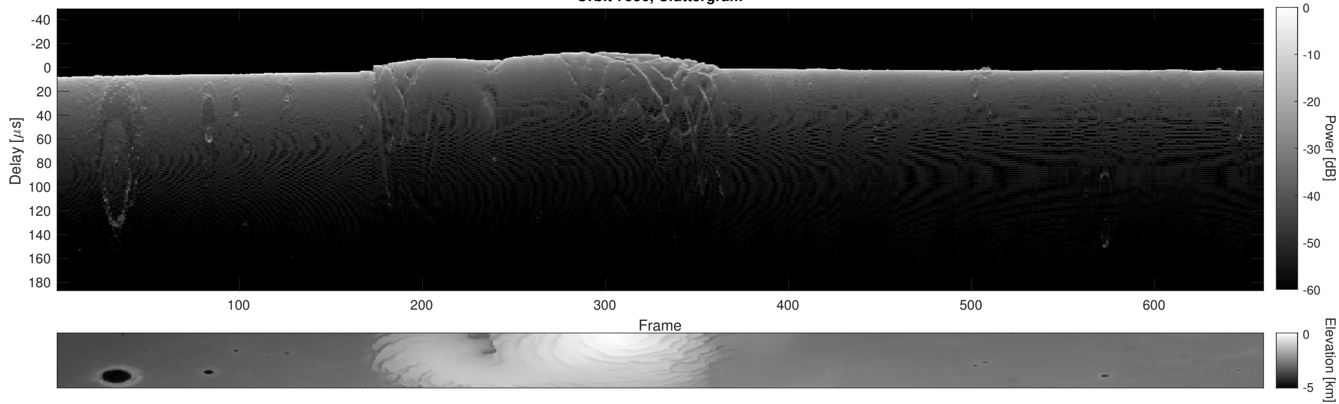
Orbit 7556, Cluttergram
